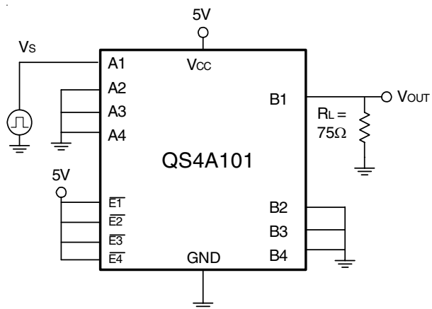
Off-Isolation
