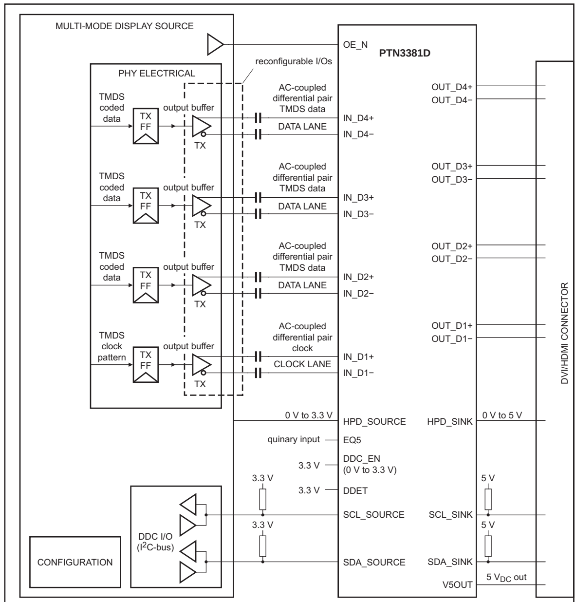
Fig 1. Typical application system diagram
