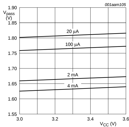
Fig 11. Pass voltage versus supply voltage; T_{amb} = 0\text{ °C} (typical)
