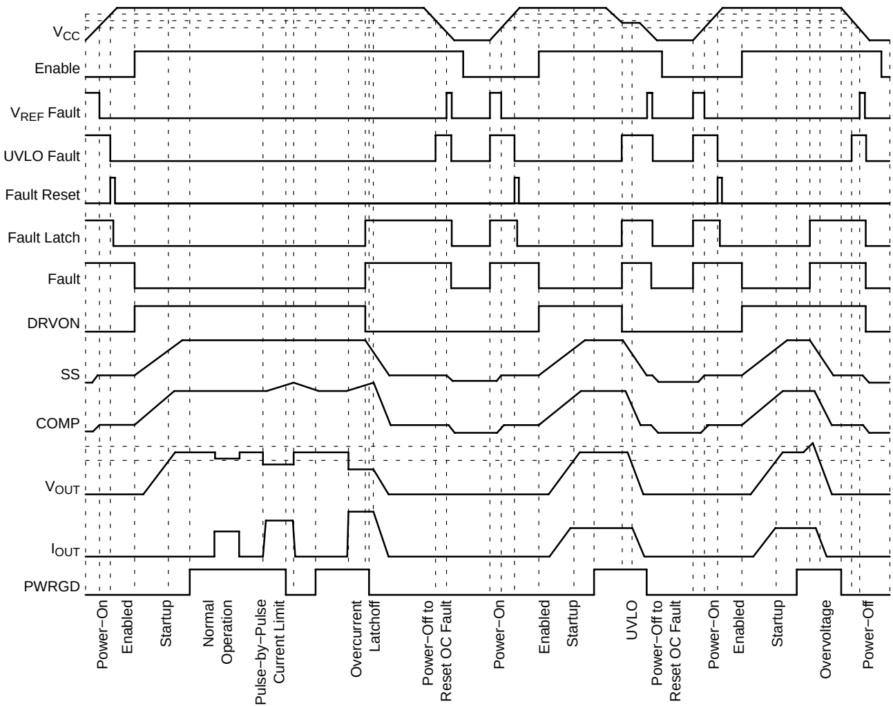
Figure 16. Operating Waveforms
