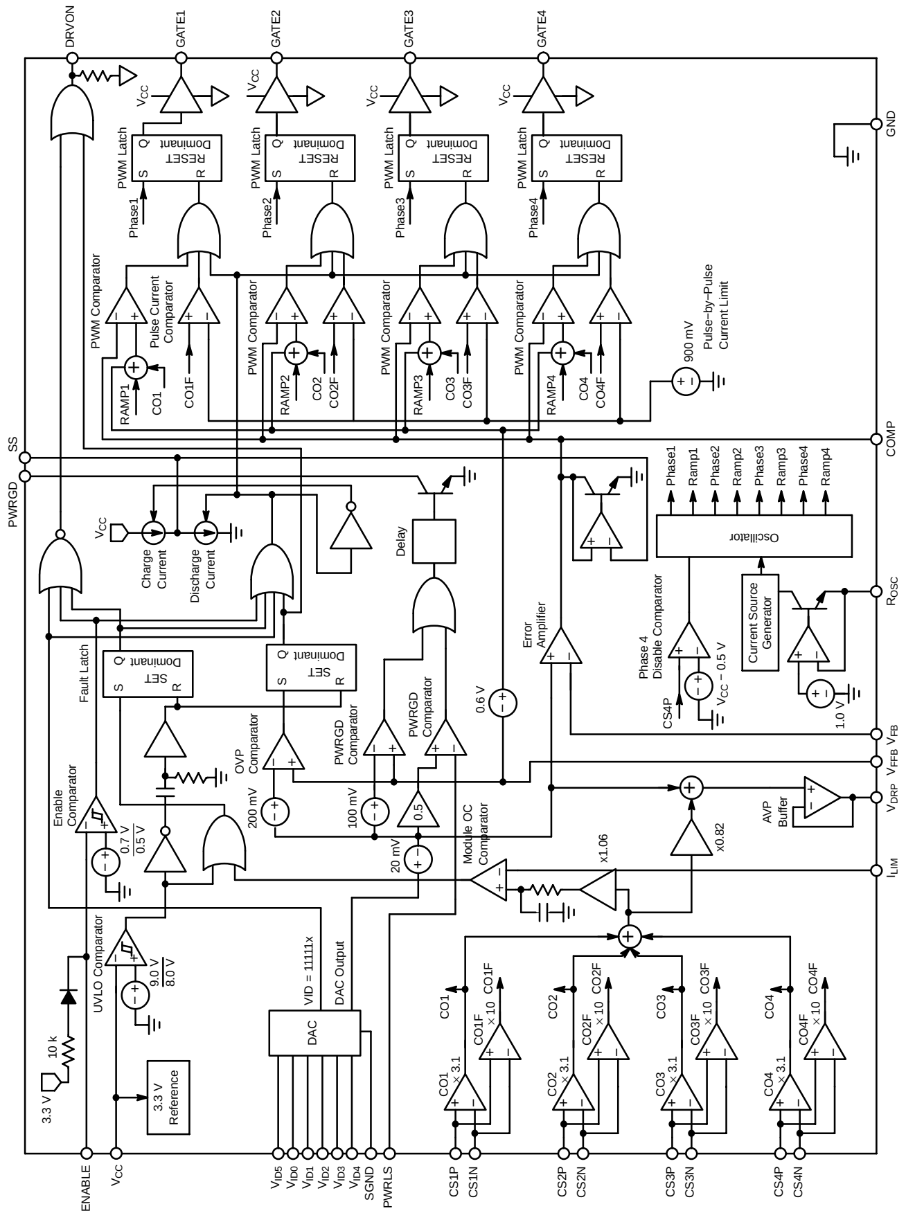
Figure 2. Block Diagram
