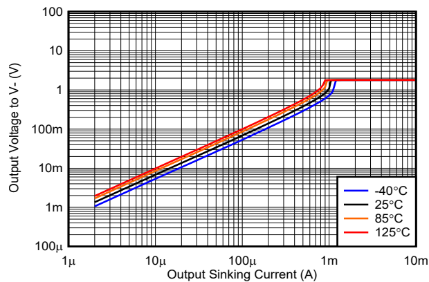
Figure 6-13. Output Voltage vs. Output Sinking Current, 1.8 V
