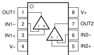
D, DGK, DDF Packages 8-Pin SOIC, VSSOP, SOT-23-8 Top View
