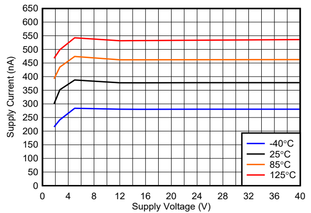
Figure 6-16. Supply Current vs. Supply Voltage (Output Low)
