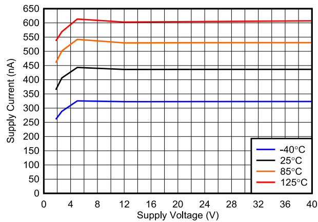
Figure 6-17. Supply Current vs. Supply Voltage (Output High)
