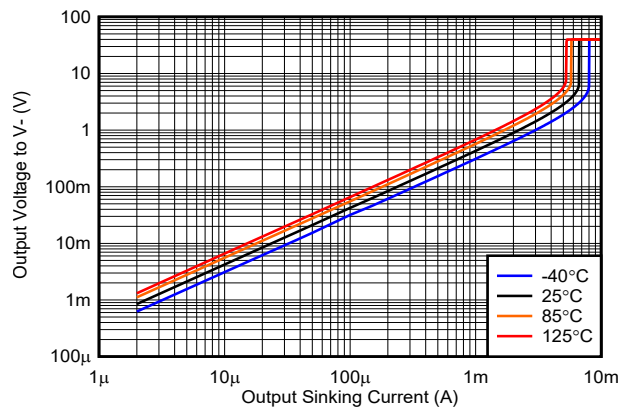
Figure 6-15. Output Voltage vs. Output Sinking Current, 40 V
