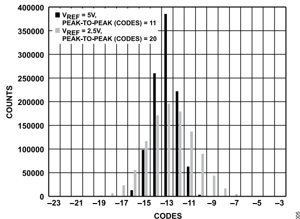
Figure 9. Histogram of a DC Input at the Code Center, V_{REF} = 2.5\text{ V} and V_{REF} = 5\text{ V}
