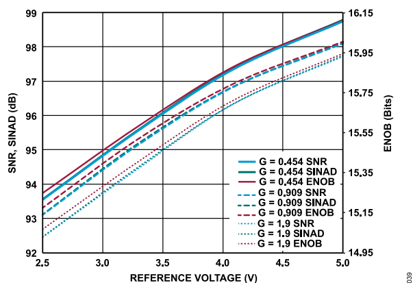
Figure 18. SNR, SINAD, and Effective Number of Bits (ENOB) vs. Reference Voltage for G = 0.454 , G = 0.909 , and G = 1.9 , f_{IN} = 1 kHz
