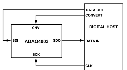
Figure 56. \overline{\text{CS}} Mode, 3-Wire Turbo Mode Connection Diagram (SDI High)
