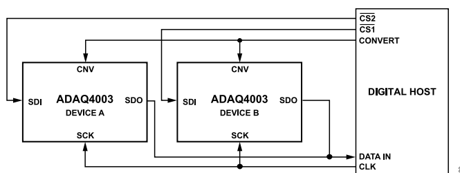
Figure 64. \overline{\text{CS}} Mode, 4-Wire Without Busy Indicator Connection Diagram
