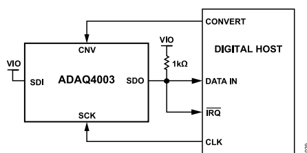
Figure 60. \overline{\text{CS}} Mode, 3-Wire with Busy Indicator Connection Diagram (SDI High)
