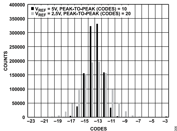
Figure 10. Histogram of a DC Input at the Code Transition, V_{REF} = 2.5\text{ V} and V_{REF} = 5\text{ V}
