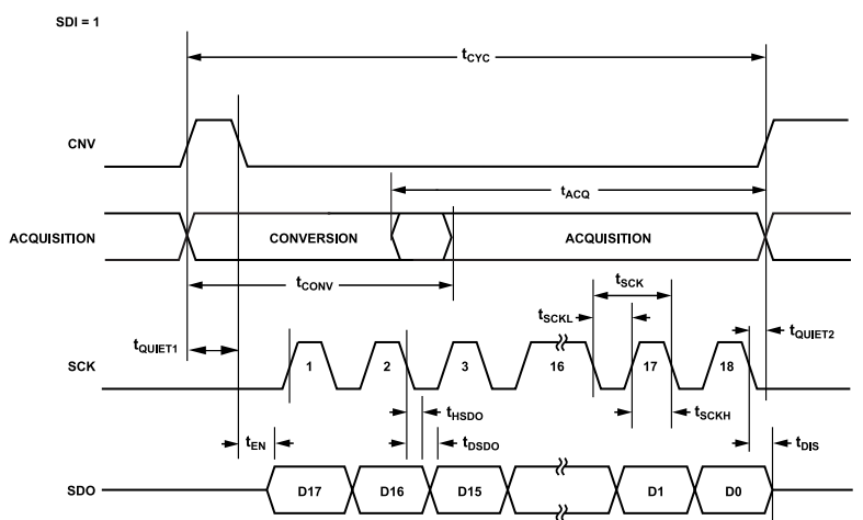
Figure 57. \overline{\text{CS}} Mode, 3-Wire Turbo Mode Serial Interface Timing Diagram (SDI High)
