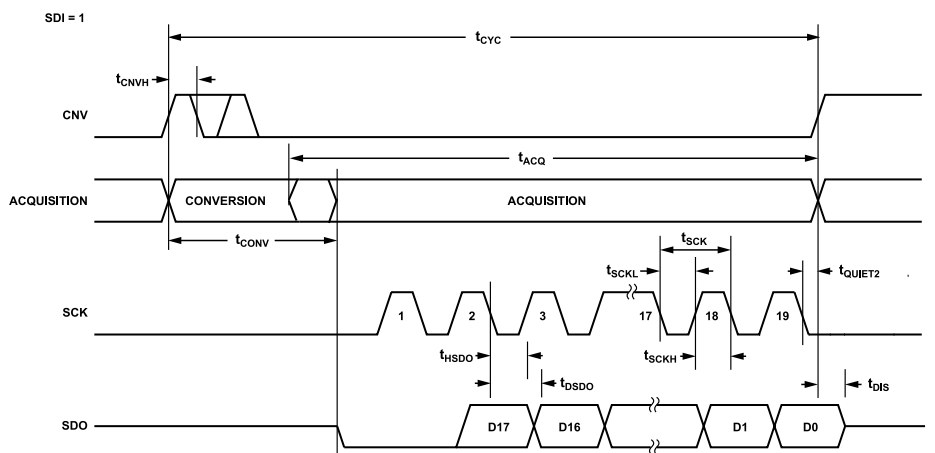
Figure 61. \overline{\text{CS}} Mode, 3-Wire with Busy Indicator Serial Interface Timing Diagram (SDI High)
