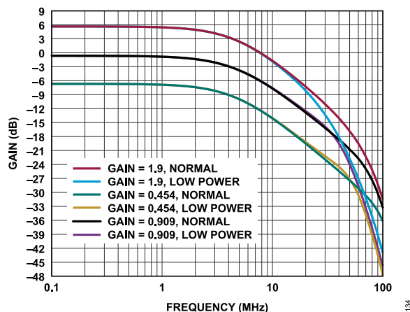
Figure 38. Small Signal Frequency Response for G = 1.9 , G = 0.454 , and G = 0.909 at Full Power and Low Power
