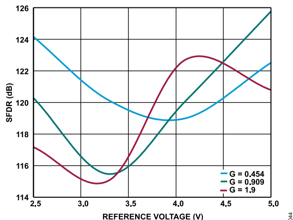
Figure 25. SFDR vs. Reference Voltage for G = 0.454 , G = 0.909 , and G = 1.9 , f_{IN} = 1 kHz
