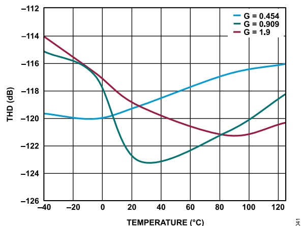
Figure 23. THD vs. Temperature for G = 0.454 , G = 0.909 , and G = 1.9 , f_{IN} = 1 kHz
