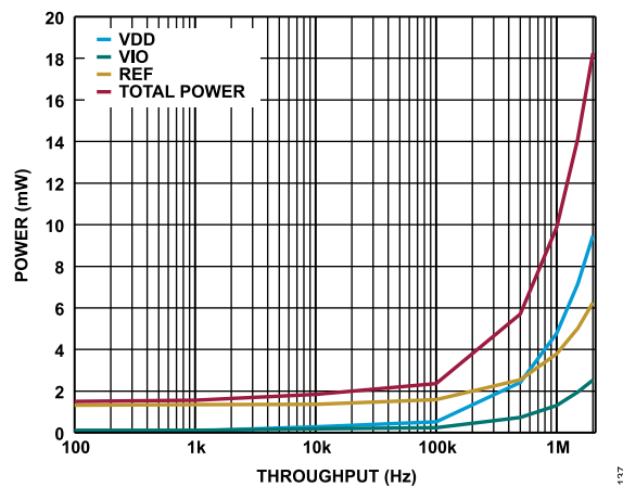
Figure 32. Power vs. Throughput
