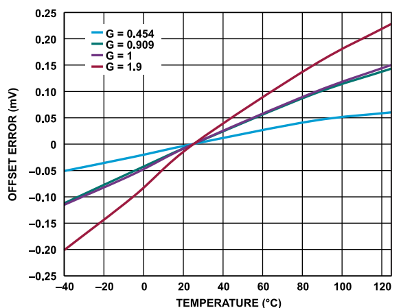
Figure 27. Offset Error vs. Temperature for G = 0.454 , G = 0.909 , G = 1 , and G = 1.9
