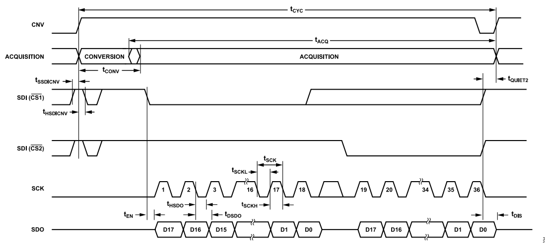
Figure 65. \overline{\text{CS}} Mode, 4-Wire Without Busy Indicator Serial Interface Timing Diagram
