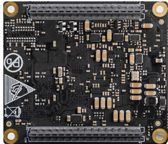
MYC-CZU3EG/4EV/5EV-V2 Bottom-view
