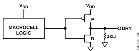
Figure 6. Data-Ready Output
