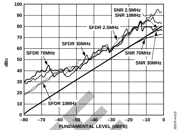
Figure 19. SFDR and SNR vs. Analog Input Level
