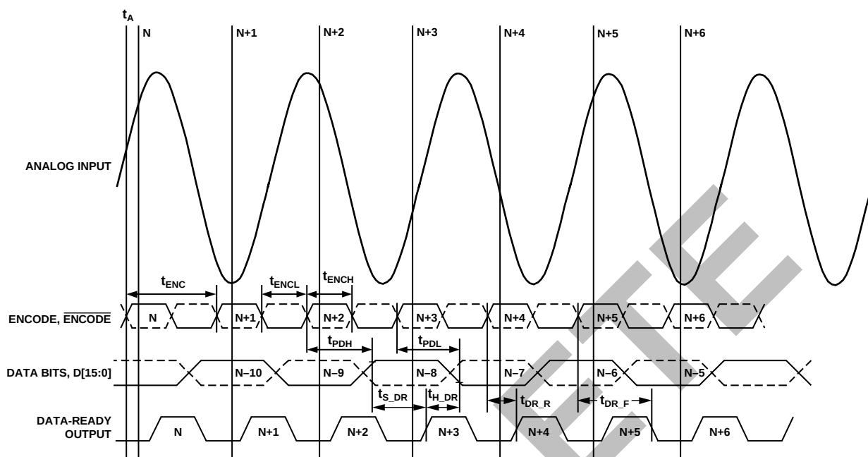
Figure 2. Timing Diagram
