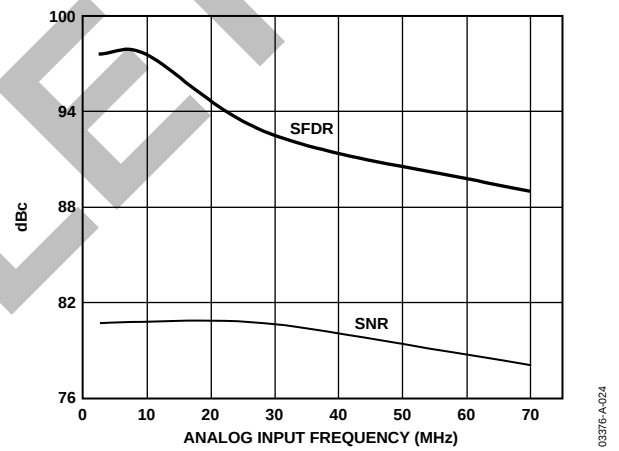
Figure 20. SFDR and SNR vs. Analog Input Frequency
