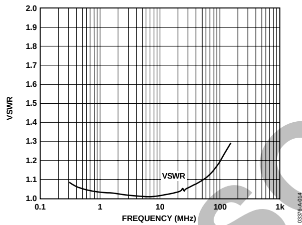
Figure 18. Analog Input VSWR
