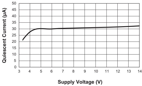
Operation Quiescent Current vs. Supply Voltage
