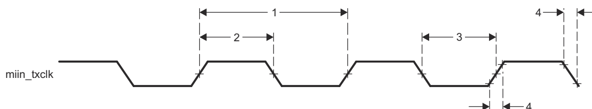
Figure 7-18. Clock Timing (GMAC Transmit) - MII operation
