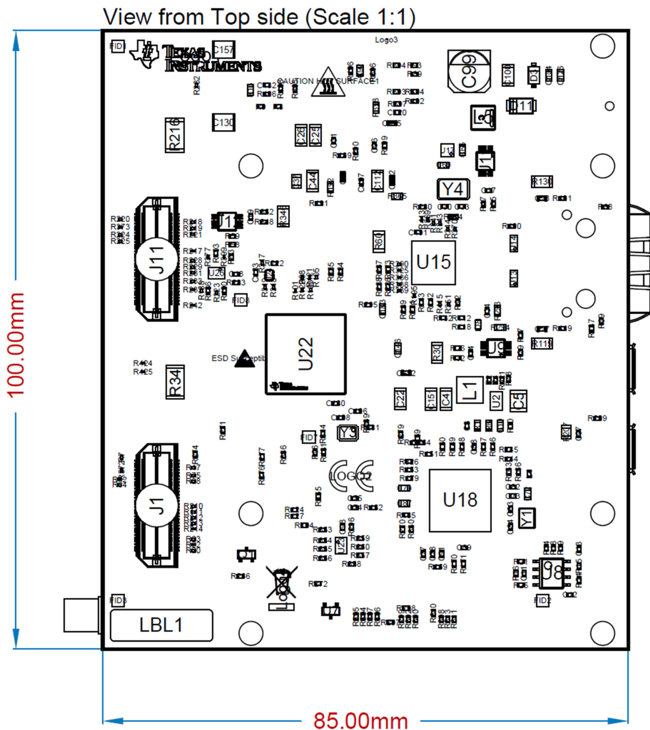
Figure 9-4. AM2732x EVM - Top Assembly
