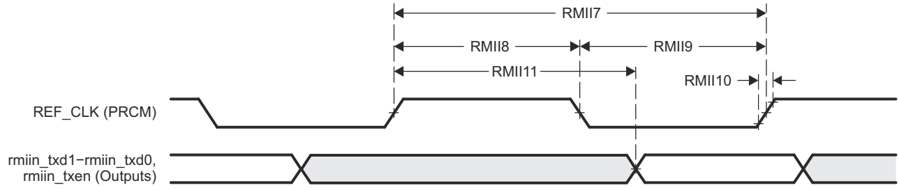
Figure 7-13. GMAC Transmit Interface Timing RMIIn Operation
