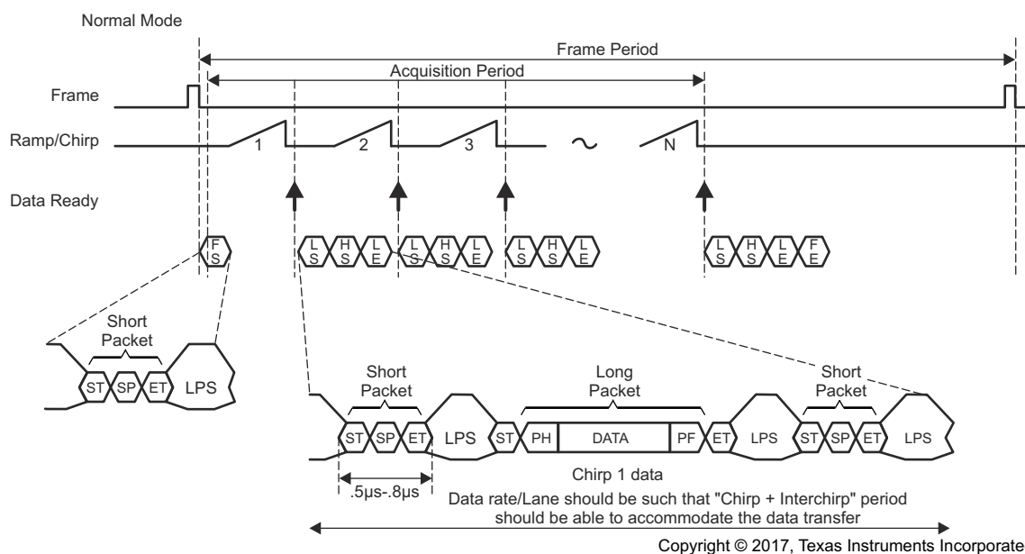
Figure 8-1. CSI-2 Transmission Format
