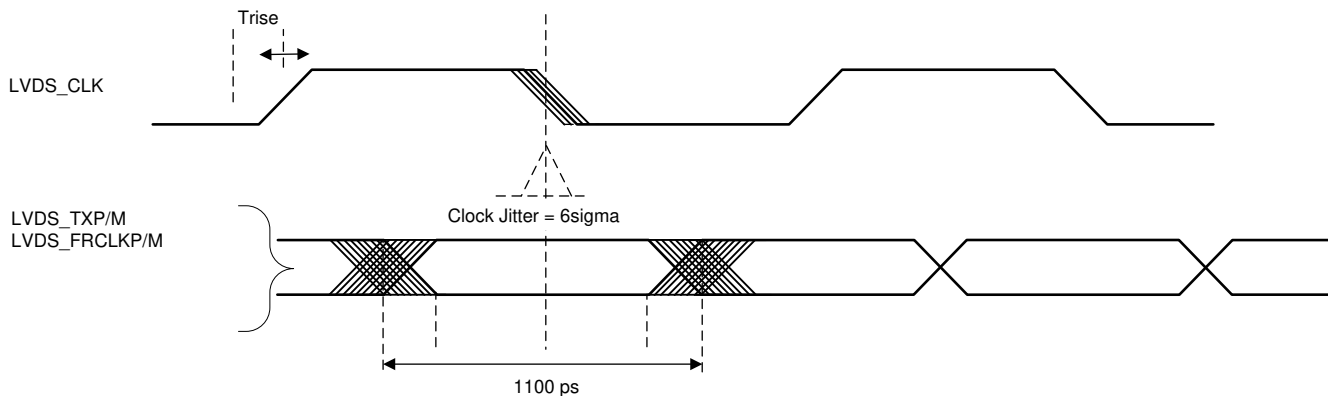
Figure 7-21. Timing Parameters
