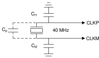
Figure 7-2. Crystal Implementation
