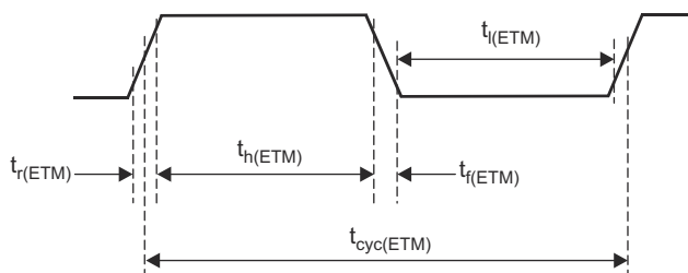
Figure 7-24. ETMTRACECLKOUT Timing
