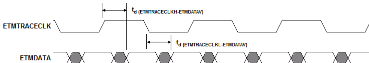
Figure 7-25. ETMDATA Timing
