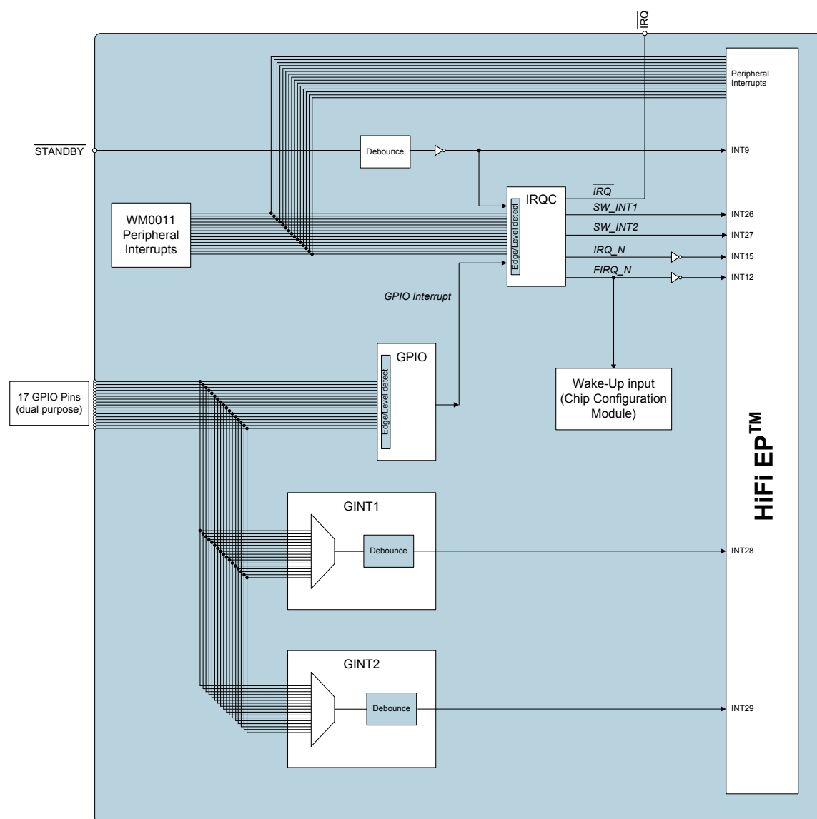
Figure 15 External and Internal Interrupts to HiFi EP™
