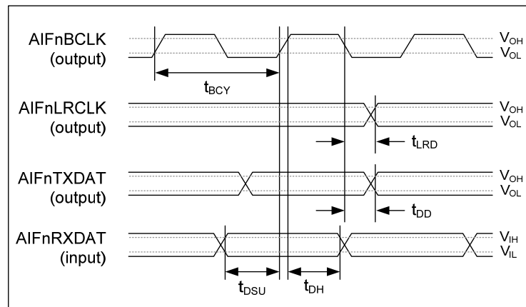
Figure 2 AIF Interface Timing – Master Mode
