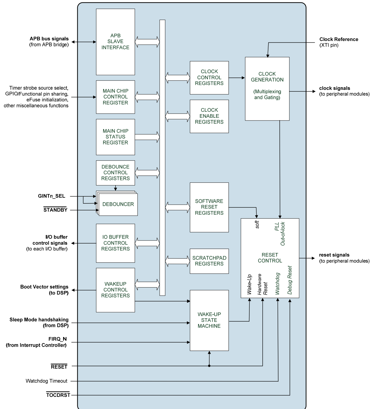
Figure 20 Chip Configuration Module (CCM) Block Diagram
