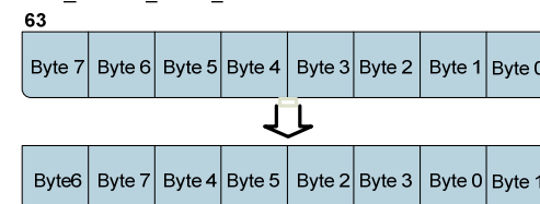
Figure 49 Endian Byte Swap
