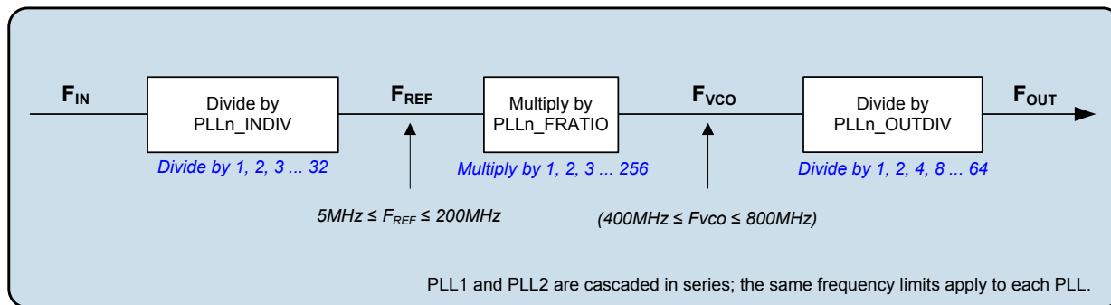
Figure 18 PLL Configuration
