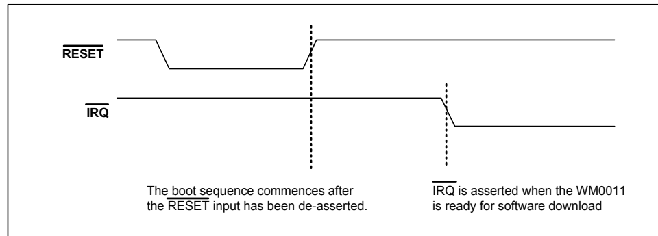
Figure 9 Hardware Reset Sequence
