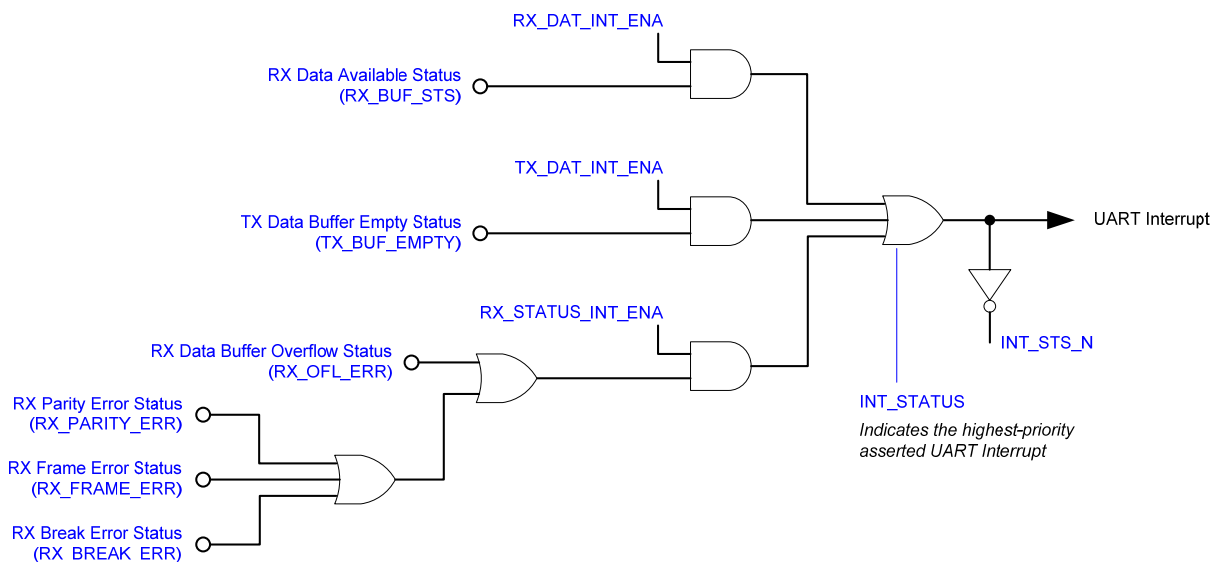
Figure 34 UART Interrupts
