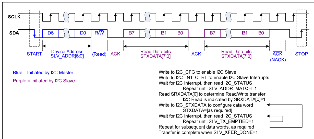
Figure 29 I2C Slave Read
