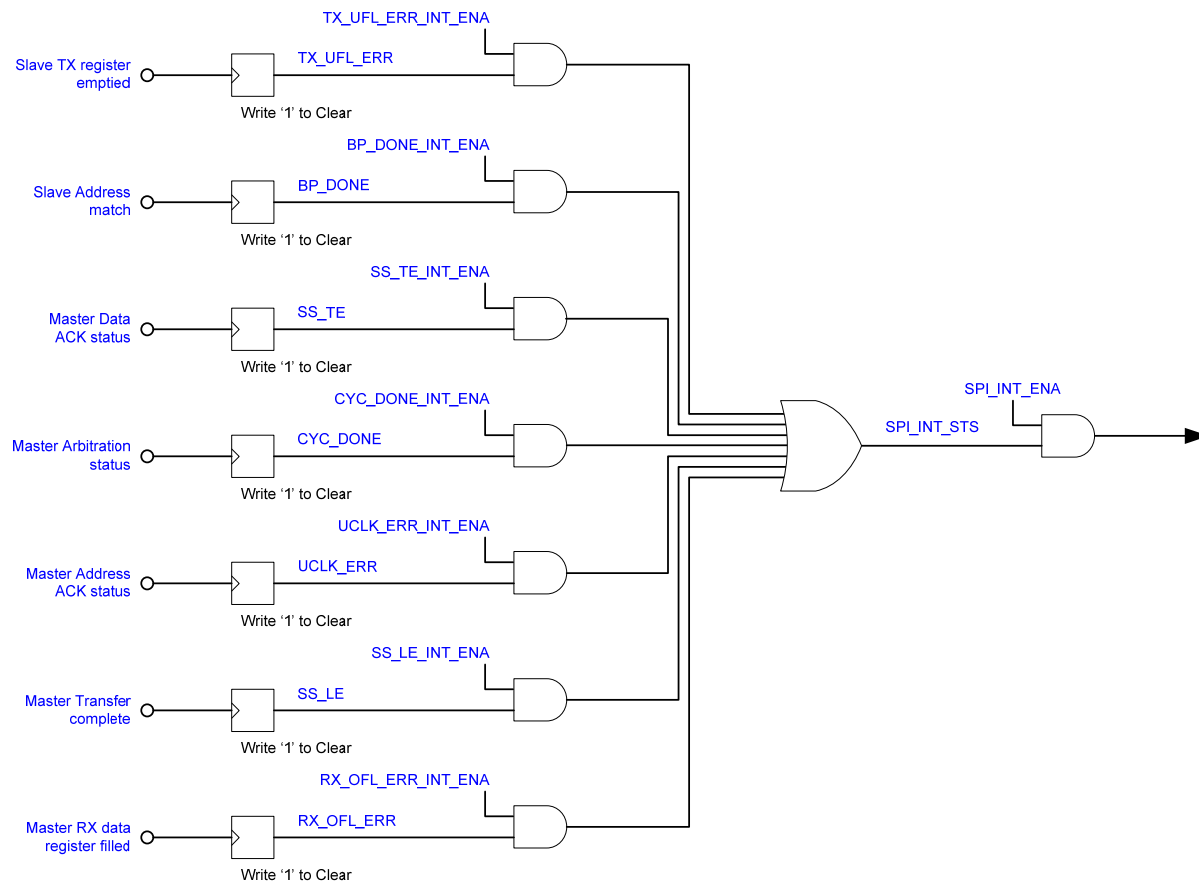
Figure 44 SPI Interrupts
