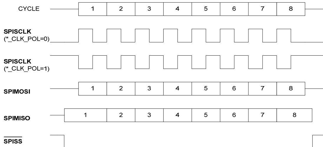
Figure 36 SPI Protocol with CLK_PHASE=1
