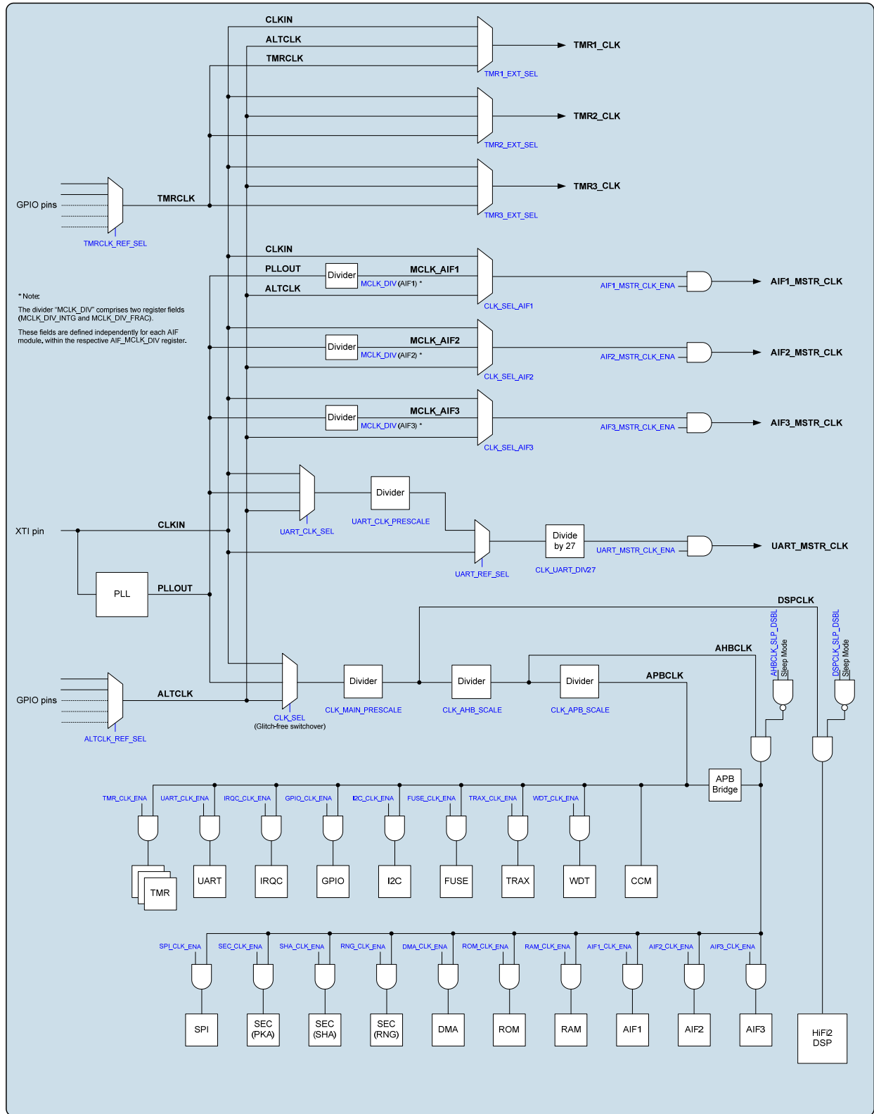
Figure 16 Clocking Architecture
