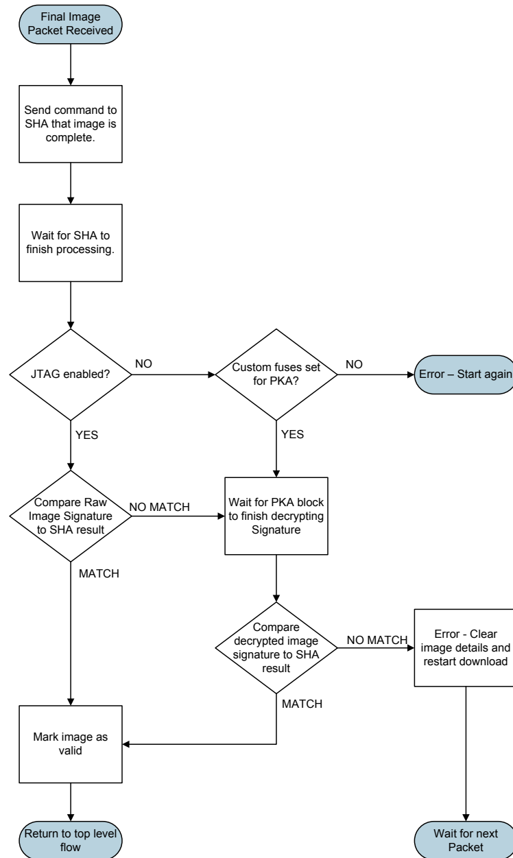
Figure 14 Application Validation
