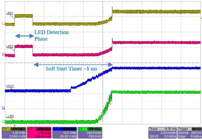
Figure 6: A80603 normal startup showing all channels passed LED Detection phase. Total LED current = 100 mA × 4 (only LED1 and LED2 pin voltages are shown).
