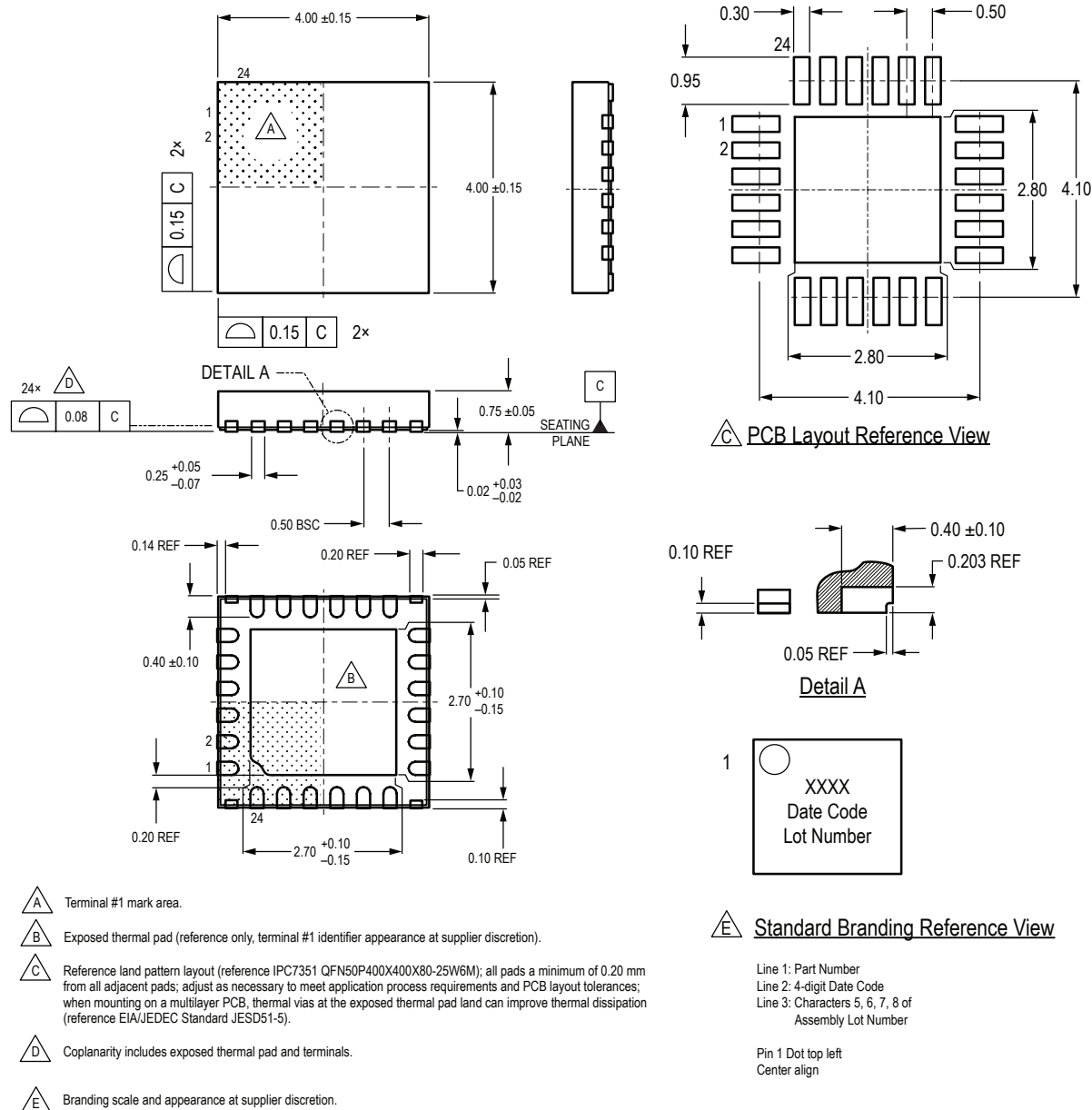
Figure 45: Package ES, 24-Pin 4 mm × 4 mm QFN with Exposed Thermal Pad and Wettable Flank
