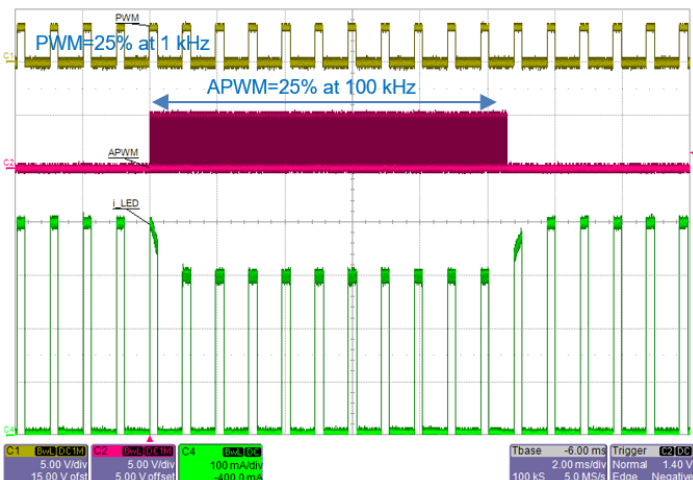
Figure 29: PWM = 25% at 1 kHz. Peak LED current drops from 400 mA ( 4 \times 100 \text{ mA/ch} ) to 300 mA when APWM of 25% duty cycle is applied
