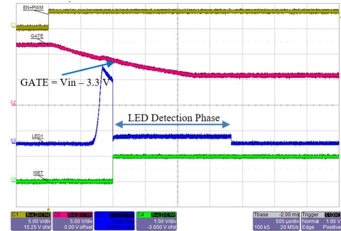
Figure 4: Startup showing EN+PWM, GATE, LED1, and ISET. Switching frequency = 2.15 MHz. Note that LED Detection Phase starts as soon as GATE pin is pulled down to 3.3 V below VIN (provided that PWM = H).
