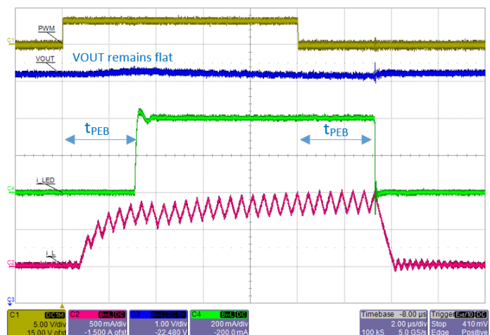
Figure 24: A80603 PWM dimming operation with PEB delay set to 3 \mu s. Note that V_{OUT} ripple is reduced to ~0.2 V.
