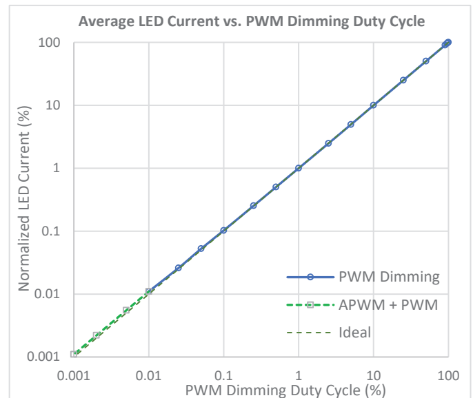
Figure 30: How to achieve 100,000:1 dimming ratio by using both PWM and APWM. Test conditions: V_{IN} = 12 \text{ V} , V_{OUT} = 25 \text{ V} ( 8 \times WLED ), total LED current = 400 mA, PWM frequency = 200 Hz, APWM frequency = 100 kHz.
