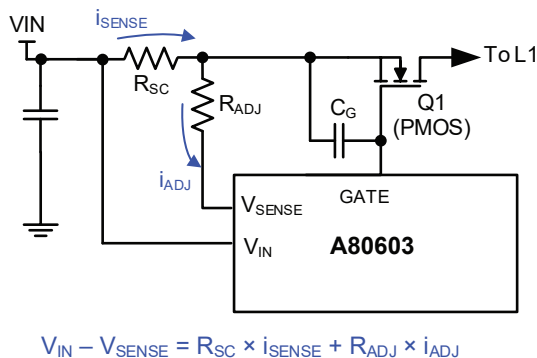
Figure 43: Optional input disconnect switch using a PMOSFET
