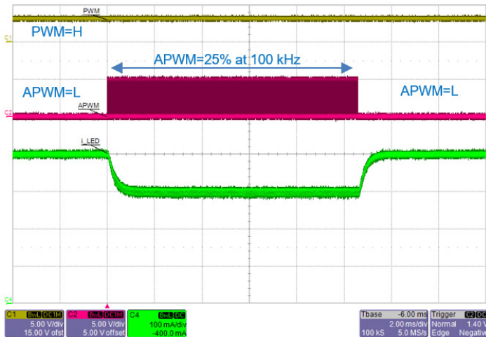
Figure 28: PWM = H. Total LED current drops from 400 mA ( 4 \times 100 \text{ mA/ch} ) to 300 mA when APWM of 25% duty cycle is applied. Note that LED current takes \sim 0.5 \text{ ms} to settle after change in APWM.
