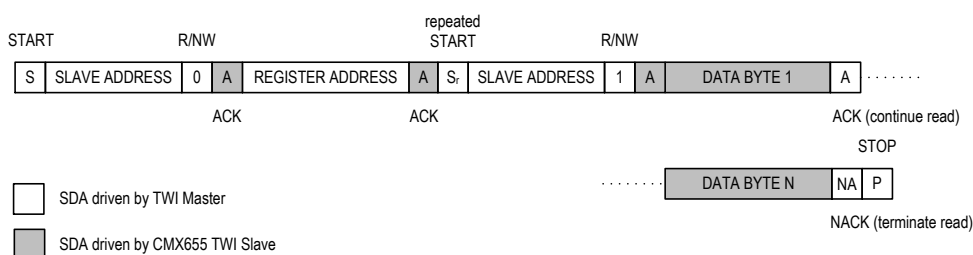
Figure 34 TWI N-Byte Read Transfer
