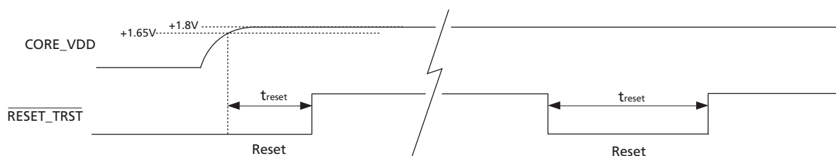
Figure 4-16: Reset Pulse
