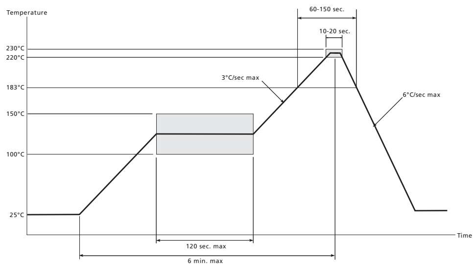
Figure 7-1: Standard Eutectic Solder Reflow Profile
