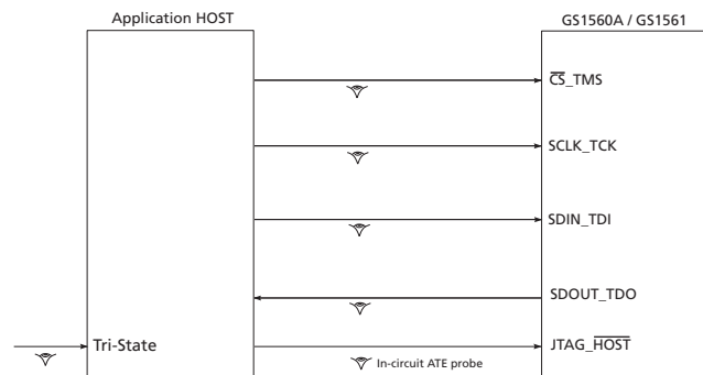
Figure 4-15: System JTAG
