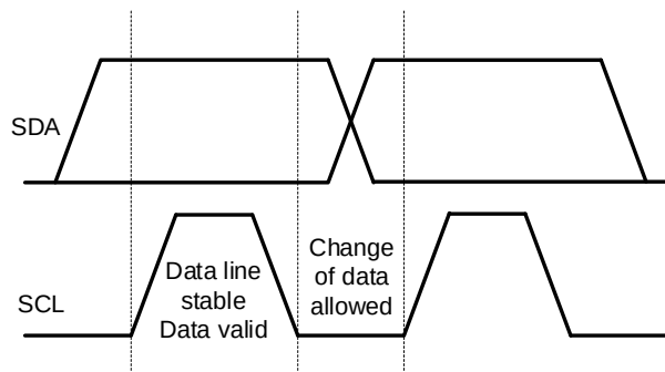
Figure 7: Bit Transfer on the I 2 C Bus
