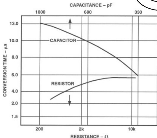
Figure 7. AD578 Conversion Times vs. R or C Values
