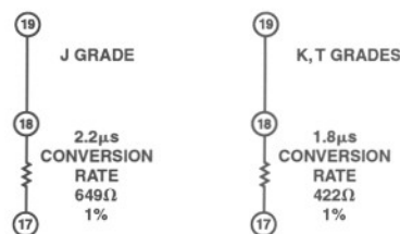
Figure 8. AD579 Clock Rate Control Connection
