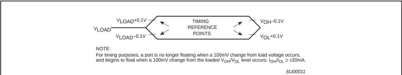
Figure 28. Float Waveform
