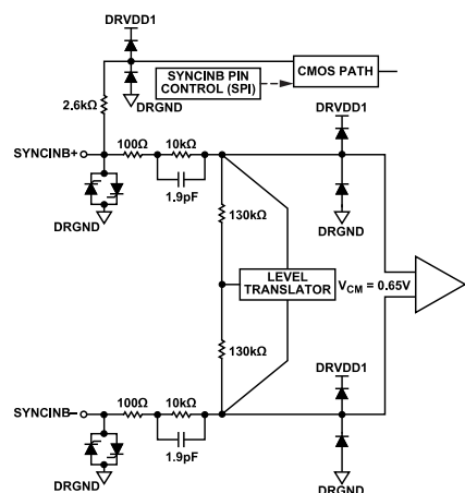
Figure 45. SYNCINB± Inputs
