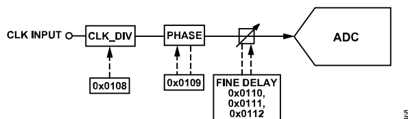
Figure 67. Clock Divider Phase and Delay Controls
