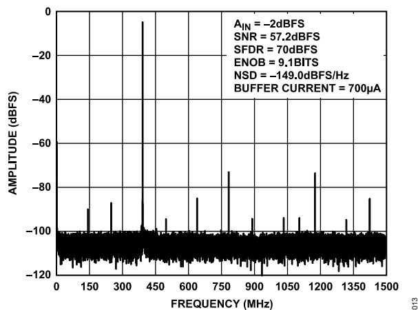
Figure 13. Single-Tone FFT at f_{IN} = 2600 MHz
