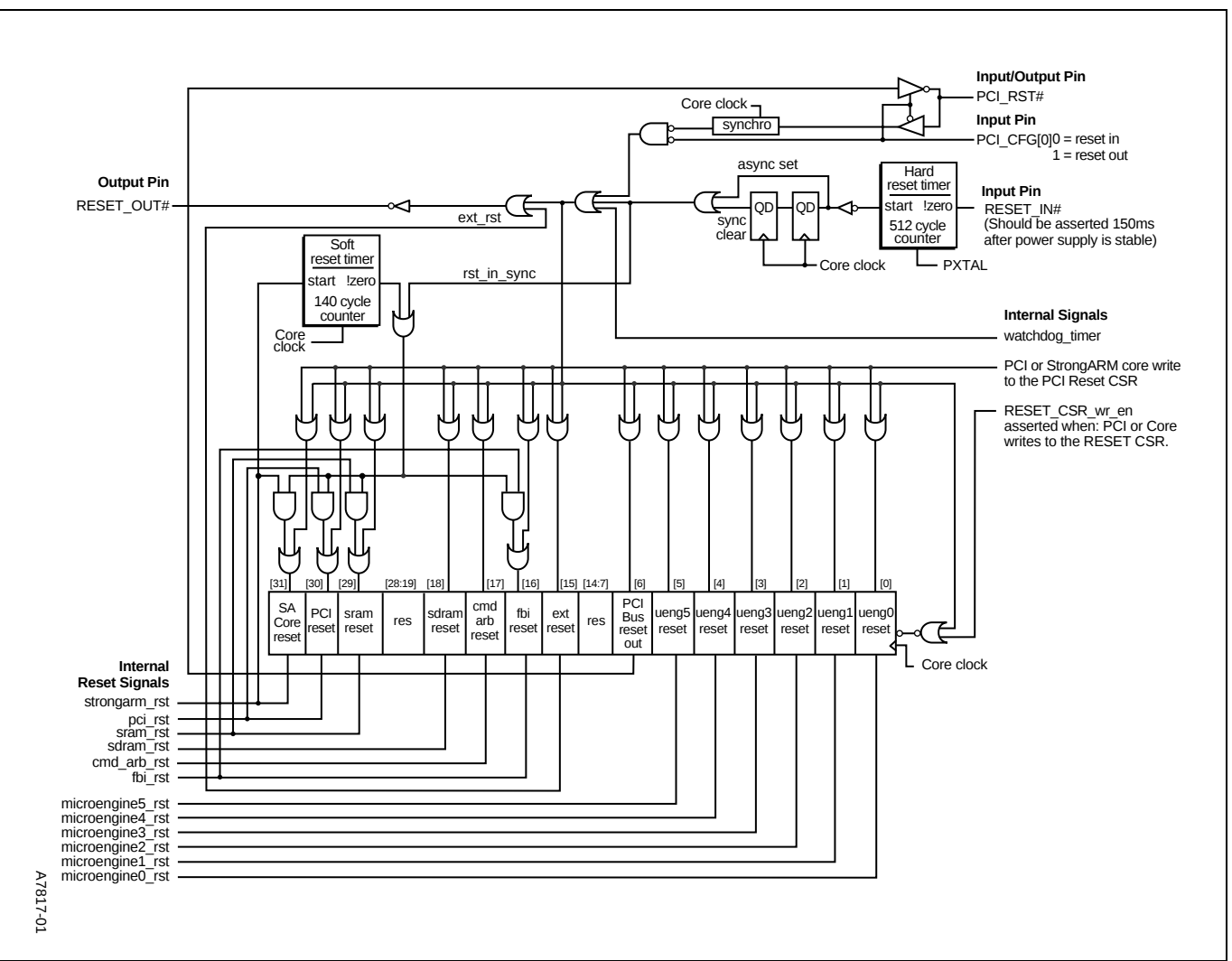
Figure 5. Reset Logic
