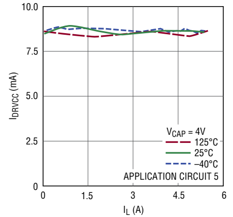
DRV CC Current vs Boost Inductor Current
