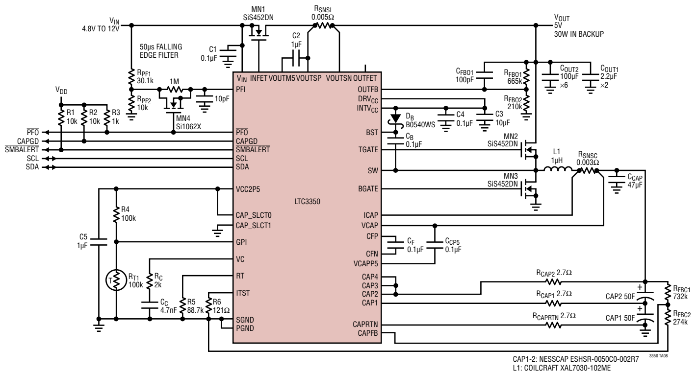
Application Circuit 7. 4.8V to 12V, 10A Supercapacitor Charger with 6.4A Input Current Limit and 5V, 30W Backup Mode
