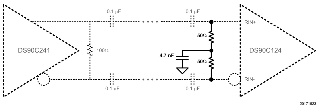
FIGURE 20. Receiver Termination Option 2
