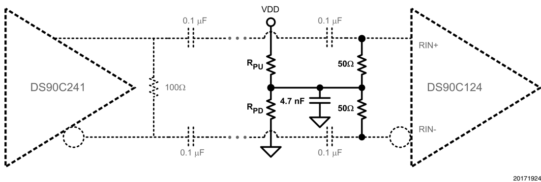
FIGURE 21. Receiver Termination Option 3
