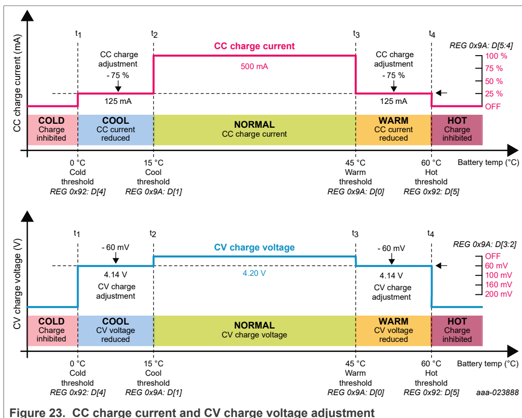
Figure 23. CC charge current and CV charge voltage adjustment
