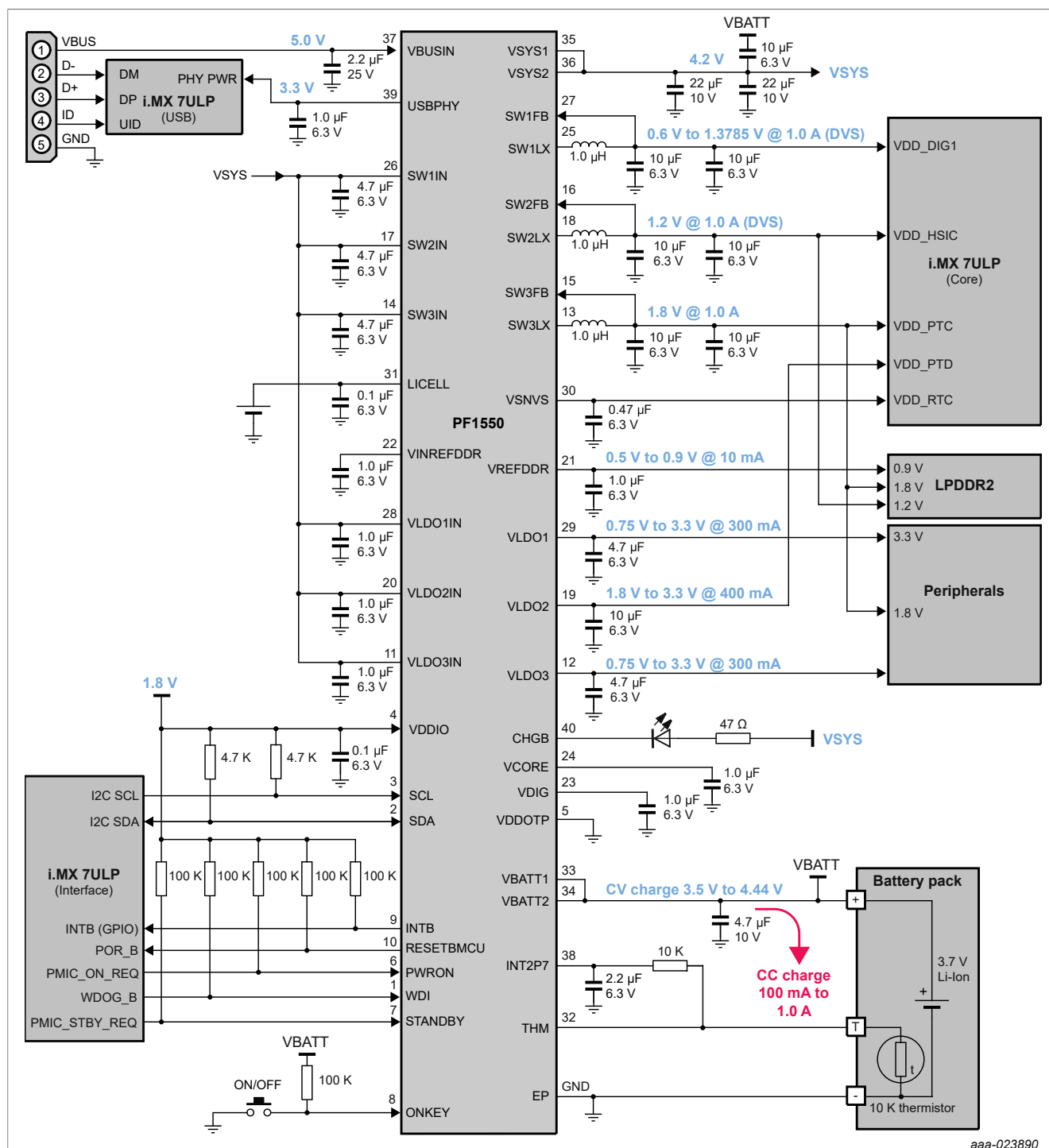
Figure 28. Typical schematic
