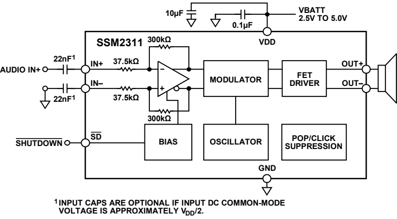
Figure 44. Single-Ended Input Configuration
