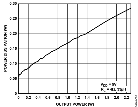
Figure 30. Power Dissipation vs. Output Power into 4 \Omega at V_{DD} = 5.0\text{ V}
