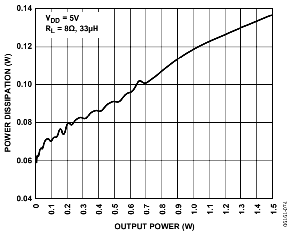
Figure 29. Power Dissipation vs. Output Power into 8 \Omega at V_{DD} = 5.0\text{ V}
