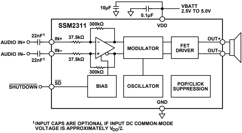
Figure 43. Differential Input Configuration
