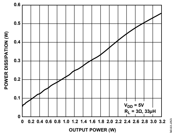
Figure 31. Power Dissipation vs. Output Power into 3 \Omega at V_{DD} = 5.0\text{ V}
