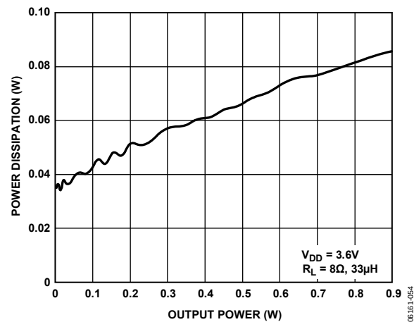
Figure 32. Power Dissipation vs. Output Power into 8 \Omega at V_{DD} = 3.6\text{ V}
