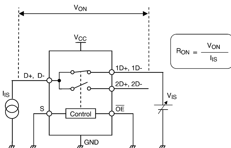
Fig. 11.9 ON-Resistance
