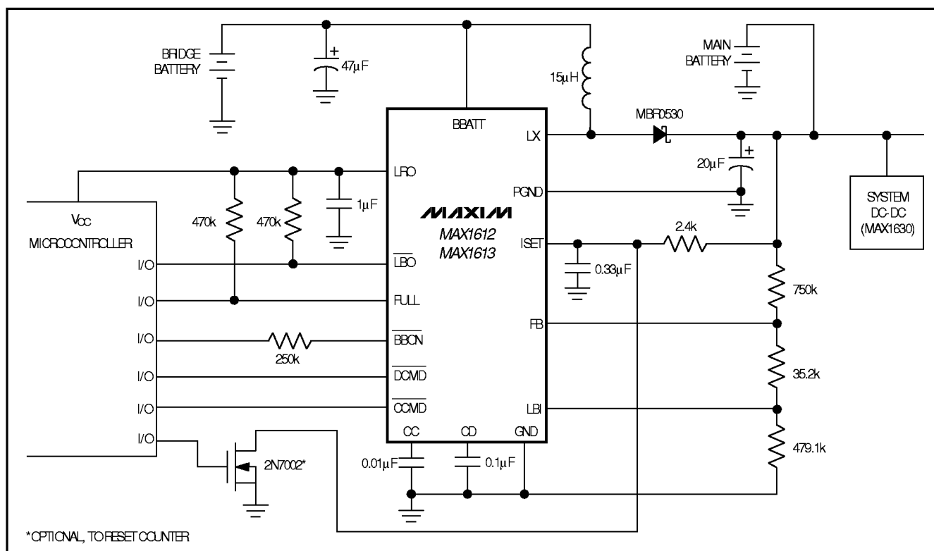
Figure 4. Microcontroller-Based Application
