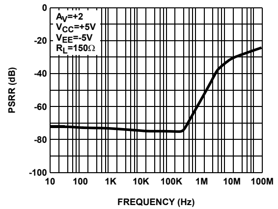
FIGURE 12. PSRR (VCC)
