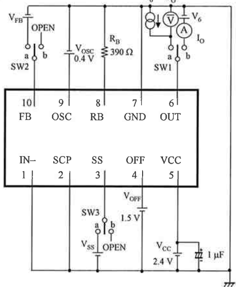
4. Test Circuit 4
