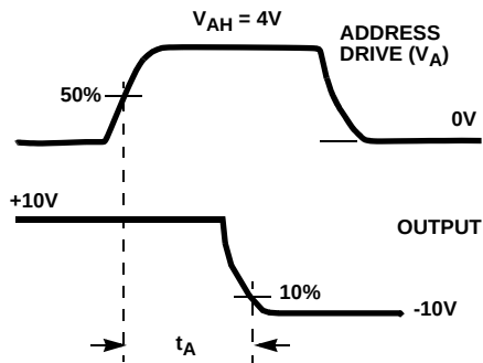
FIGURE 4C. MEASUREMENT POINTS
