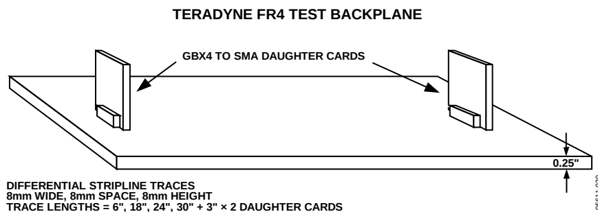
Figure 30. Test Backplane
