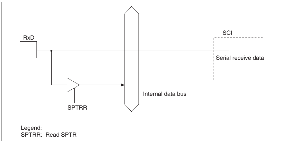
Figure 15.4 RxD Pin
