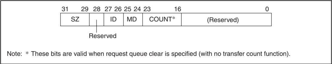
Figure 14.54 DTR Format (Transfer Request Format) (SH7751R)
