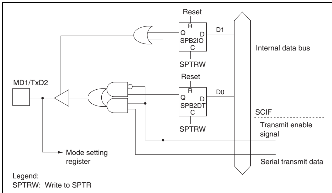
Figure 16.4 MD1/TxD2 Pin
