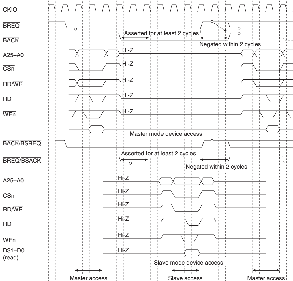
Figure 13.69 Arbitration Sequence
