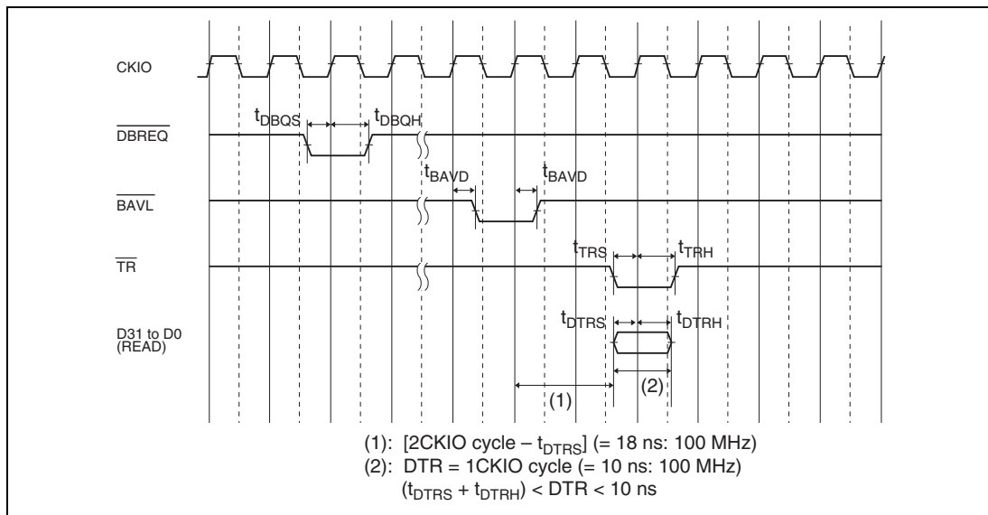
Figure 23.64 (b) \overline{\text{DBREQ}}/\text{TR} Input Timing and \overline{\text{BAVL}} Output Timing
