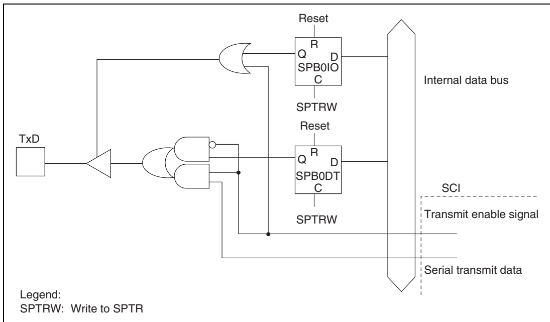
Figure 15.3 TxD Pin
