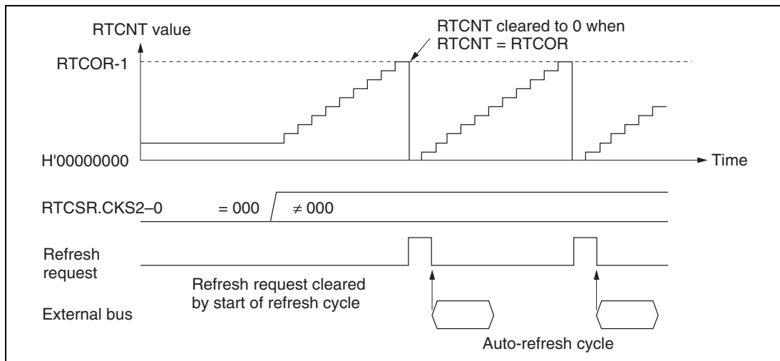
Figure 13.35 Auto-Refresh Operation
