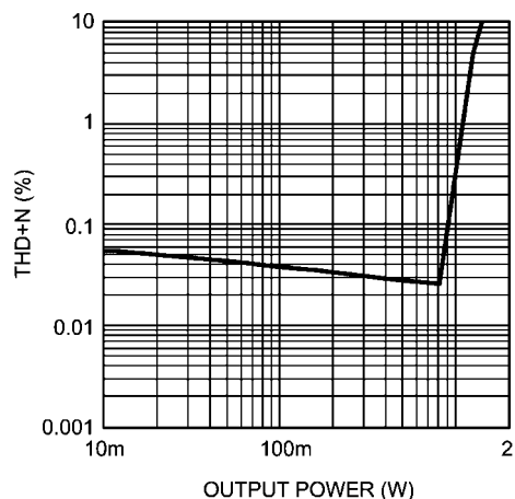
THD+N vs Output Power AV_{DD} = 5.0V , LS Out, R_L = 8\Omega , f = 1kHz
