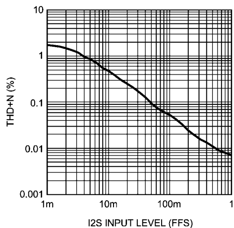
THD+N vs I²S Level EP Out
