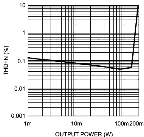
THD+N vs Output Power AV_{DD} = 5.0V , EP Out, R_L = 16\Omega , f = 1kHz
