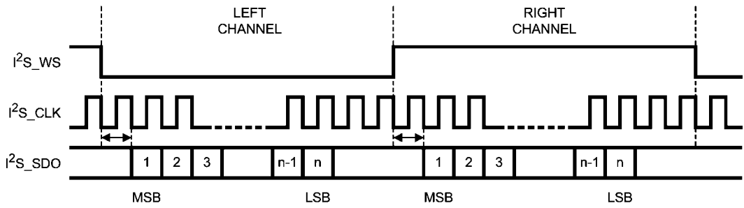
I²S Mode Timing
