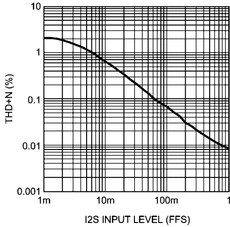
THD+N vs I 2 S Level HP Out
