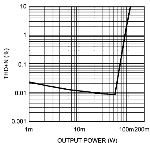
THD+N vs Output Power AV_{DD} = 5.0V , HP Out, R_L = 32\Omega , f = 1kHz
