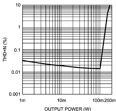
THD+N vs Output Power AV_{DD} = 5.0V , HP Out, R_L = 16\Omega , f = 1kHz
