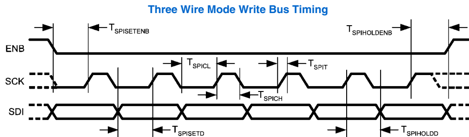
Three Wire Mode Write Bus
