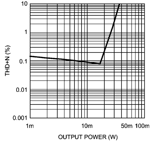
THD+N vs Output Power AV_{DD} = 3.0V , EP Out, R_L = 16\Omega , f = 1kHz
