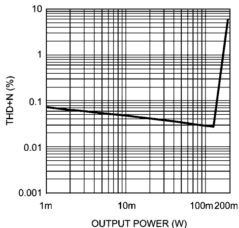
THD+N vs Output Power AV_{DD} = 5.0V , EP Out, R_L = 32\Omega , f = 1kHz
