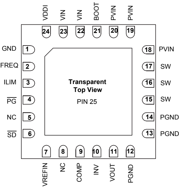
Figure 3. 34713 Pin Connections
