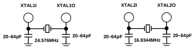
Figure 23. Crystal Connections
