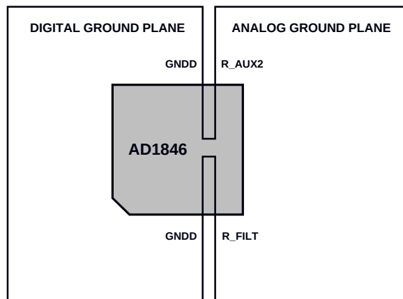
Figure 25. Recommended Ground Plane
