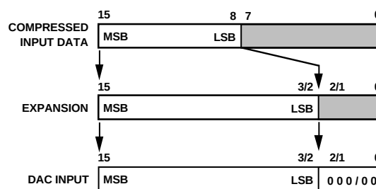
Figure 2. A-Law or \mu -Law Expansion
