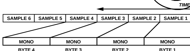
Figure 7. 8-Bit Mono Data Stream Sequencing
