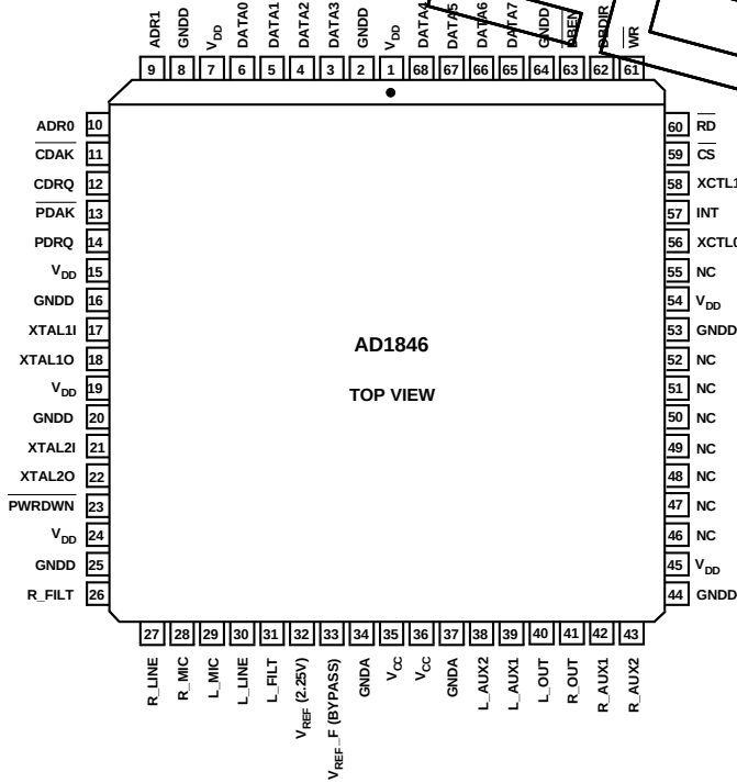
68-Lead Plastic Leaded Chip Carrier Pinout
