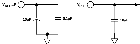
Figure 21. Voltage Reference Bypassing
