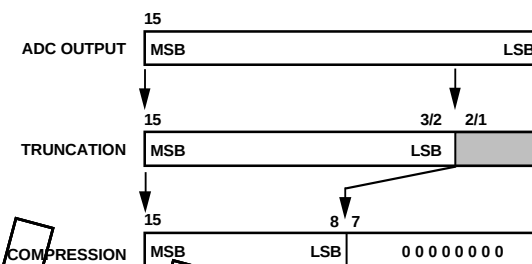
Figure 3. A-Law or \mu -Law Compression
