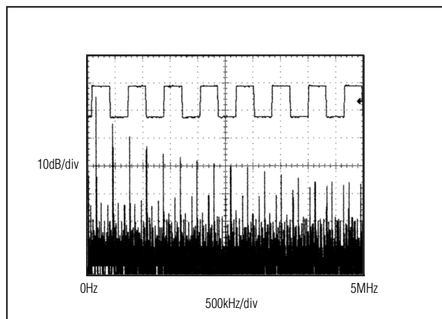
Figure 12. Driver Output Waveform and FFT Plot of MAX481/MAX483/MAX485 Transmitters Transmitting a 150kHz Signal
