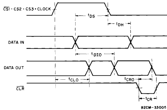
Fig. 5 - Timing waveforms for CDP1875C (output port).
