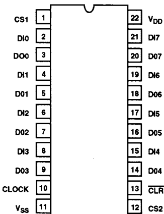
CDP1874C INPUT PORT TOP VIEW
