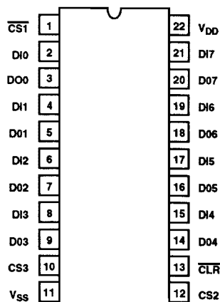
CDP1875C OUTPUT PORT TOP VIEW
