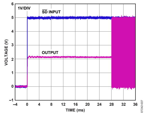
Figure 37. Turn-On Response
