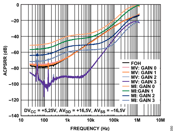
Figure 49. ACPSRR of AV_{SS} vs. Frequency
