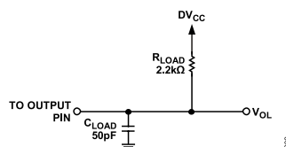
Figure 2. Load Circuit for Open Drain
