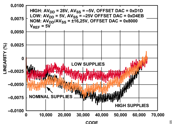
Figure 12. Measure Current Linearity vs. Code (MEASOUT Gain = 1, MI Gain = 20, T_J = 25^\circ\text{C} )
