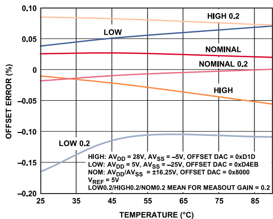
Figure 22. MI Offset Error vs. Temperature, MI Gain = 20, MEASOUT Gain = 1 and 0.2
