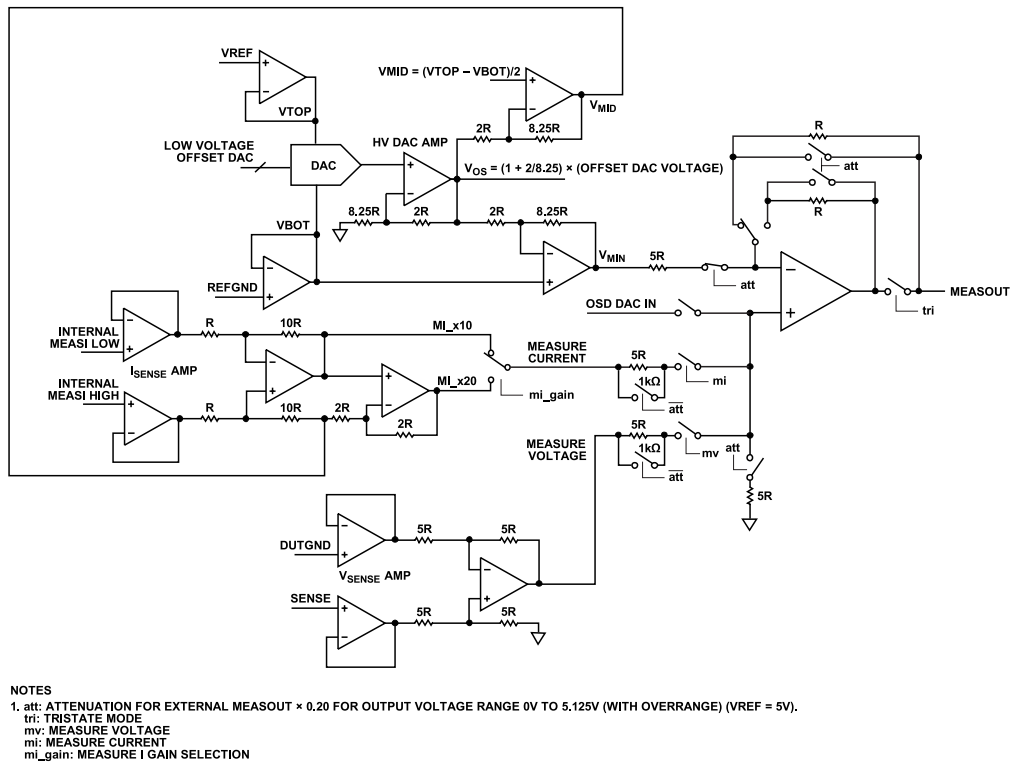
Figure 56. MI, MV, and MEASOUT Block Showing Gain Settings and Offset DAC Influence
