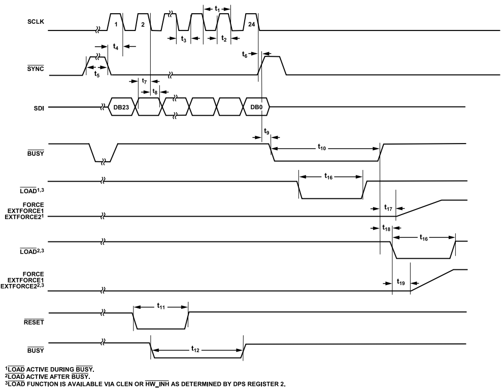
Figure 4. SPI Write Timing
