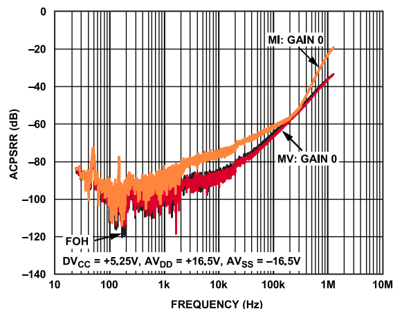
Figure 52. ACPSRR of HCAV_{SSx} vs. Frequency
