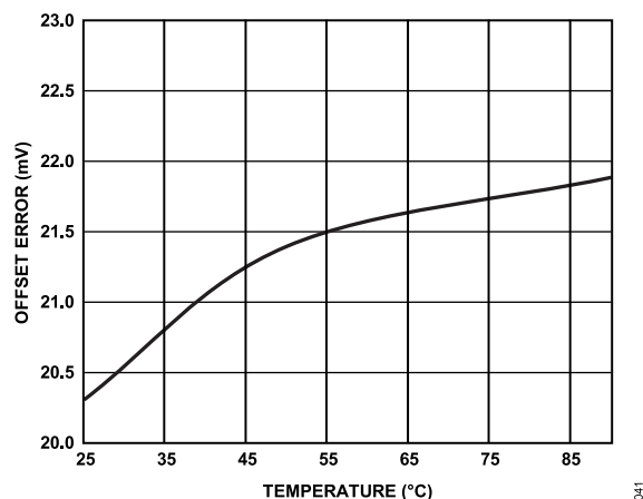
Figure 25. FV Offset Error vs. Temperature
