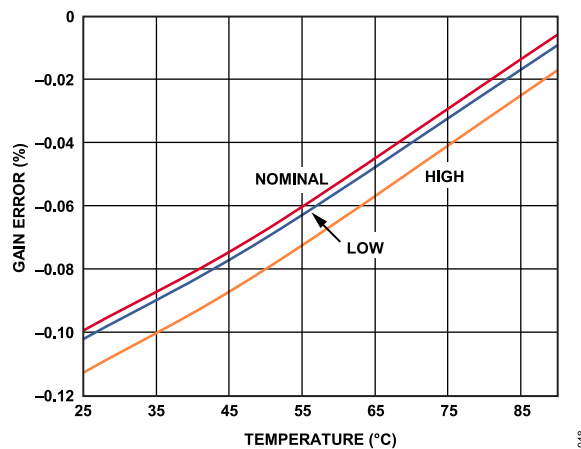
Figure 23. MI Positive Gain Error vs. Temperature, MI Gain = 20, MEASOUT Gain = 1
