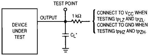
Figure 4. Test Circuit
