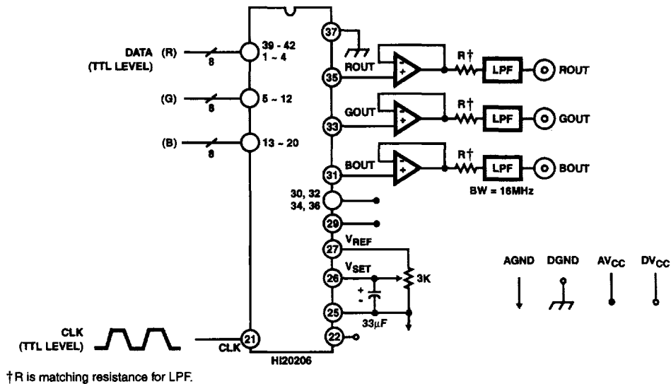
FIGURE 6. GLITCH ENERGY TEST CIRCUIT
