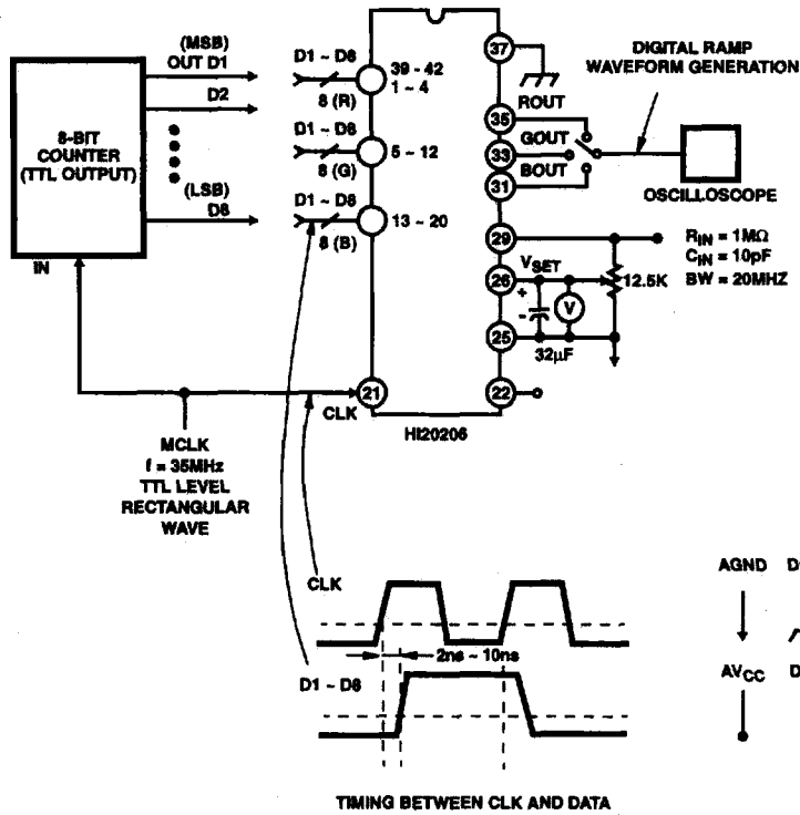
FIGURE 2. MAXIMUM CONVERSION RATE TEST CIRCUIT
