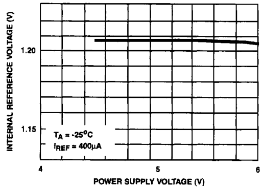
FIGURE 19. INTERNAL REFERENCE VOLTAGE vs POWER SUPPLY VOLTAGE
