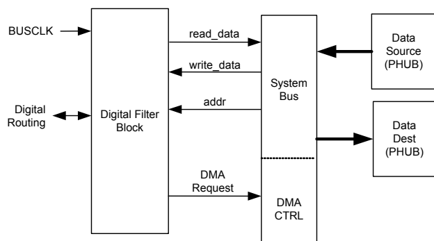
Figure 7-21. DFB Application Diagram (pwr/gnd not shown)
