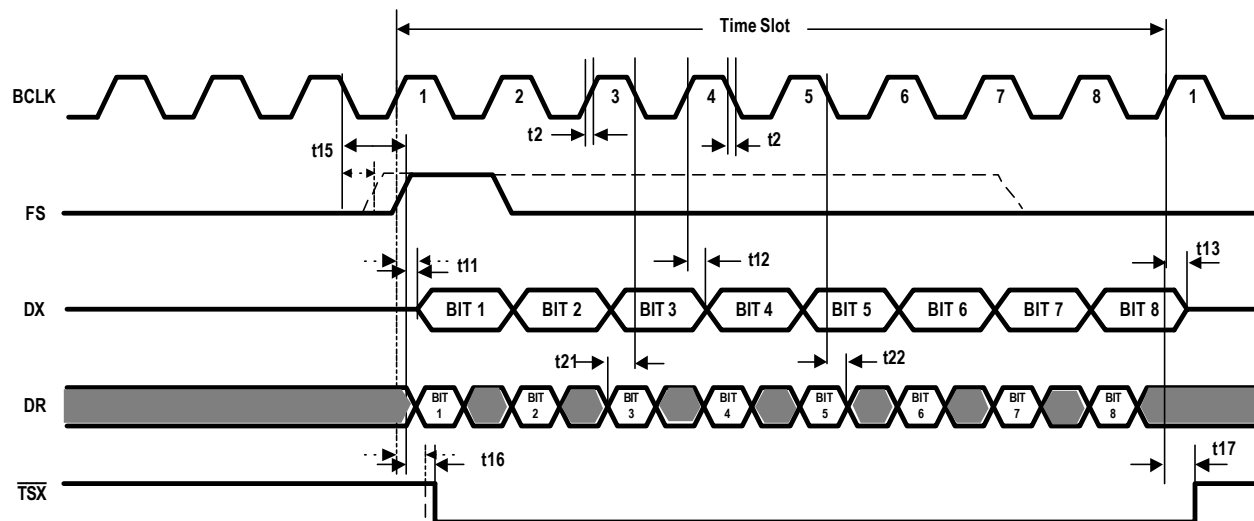
Figure 8. Transmit and Receive Timing in Non-Delay Mode
