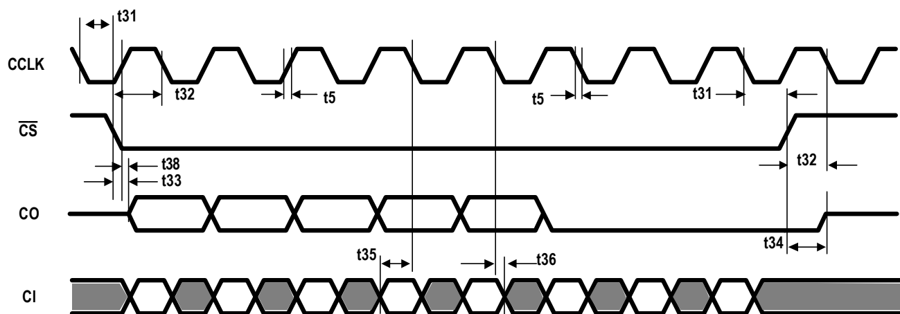
Figure 12. Serial Control Interface Timing
