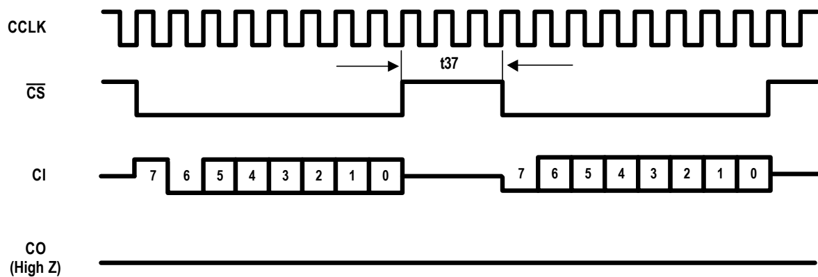
Figure 11. CODEC Programming Mode Timing
