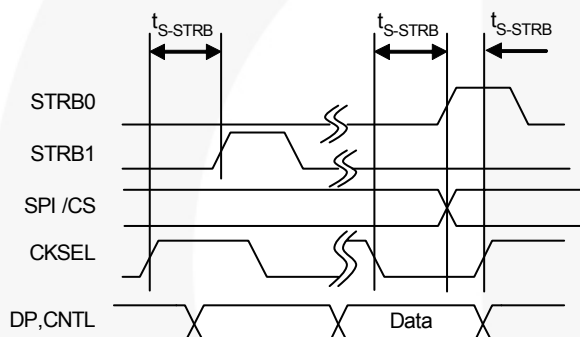
Figure 13. CKSEL Write Setup Time
