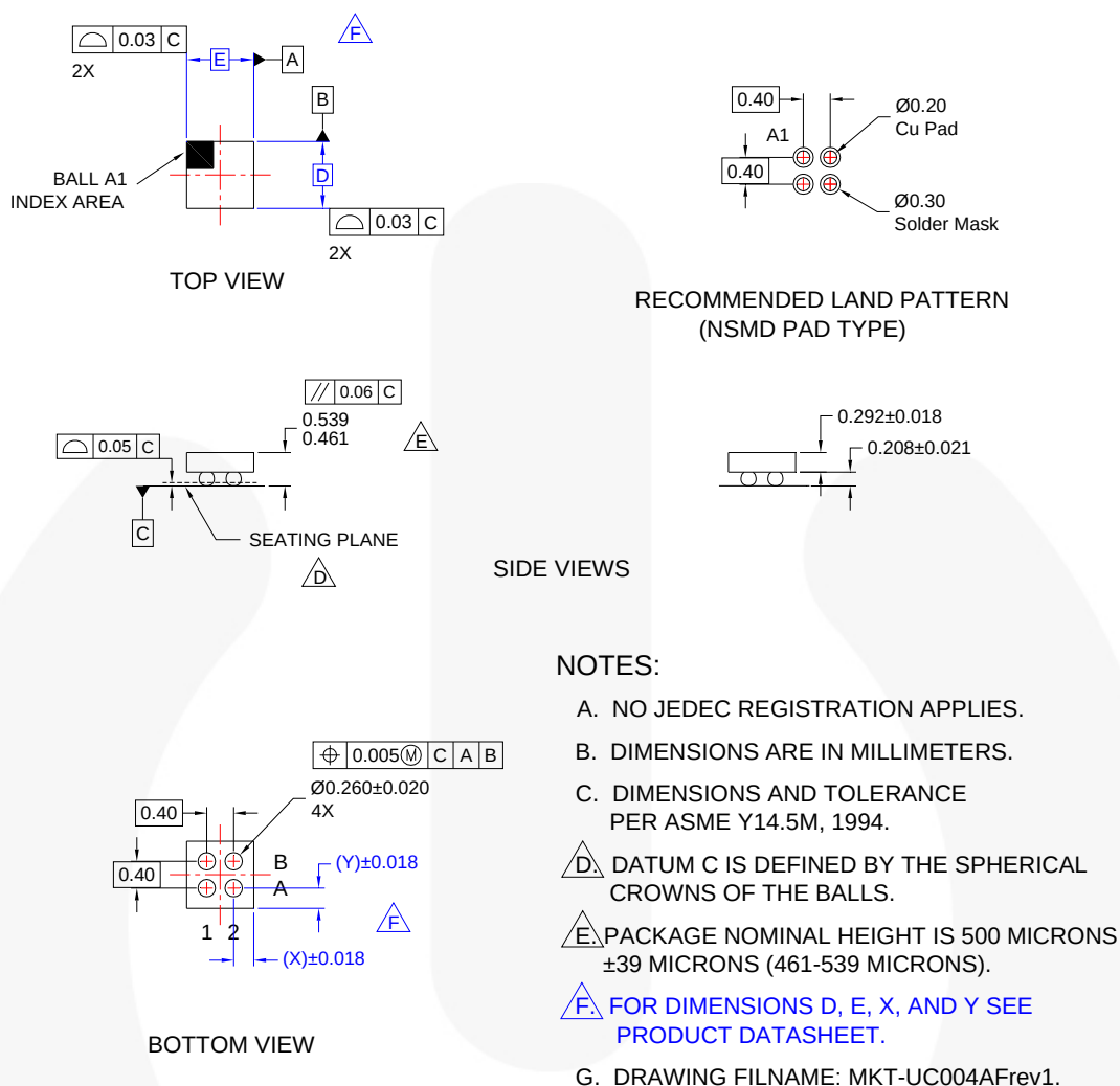
Figure 5. 4-Lead, Wafer-Level Chip Scale 0.76x0.76x0.5mm Wafer-Level Chip-Scale Package (WLCSPP)
