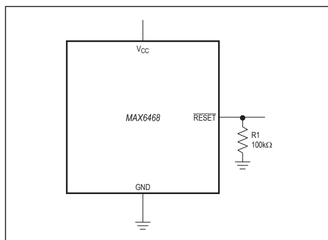
Figure 3. \overline{RESET} Valid to V_{CC} = 0V
