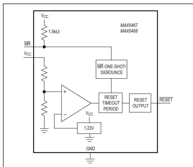
Figure 2. Functional Diagram
