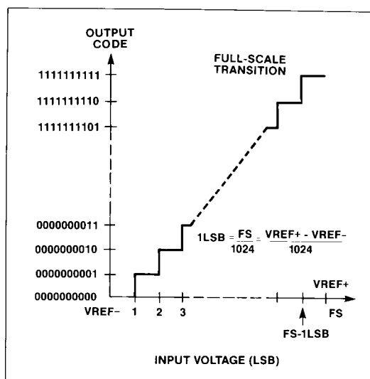
Figure 9. Ideal Transfer Function
