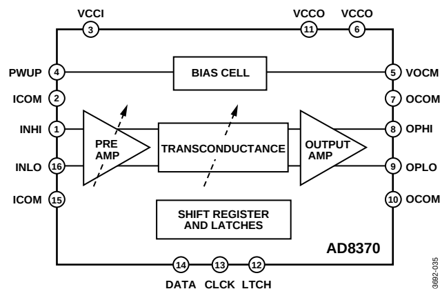
Figure 37. Functional Block Diagram
