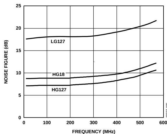
Figure 9. Noise Figure vs. Frequency at Various Gains
