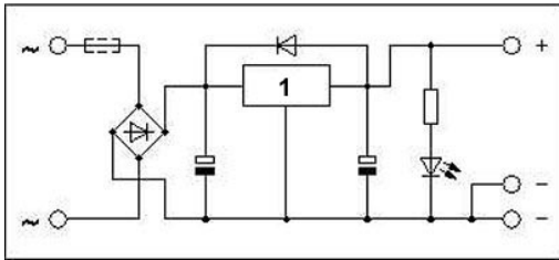
Circuit diagram
