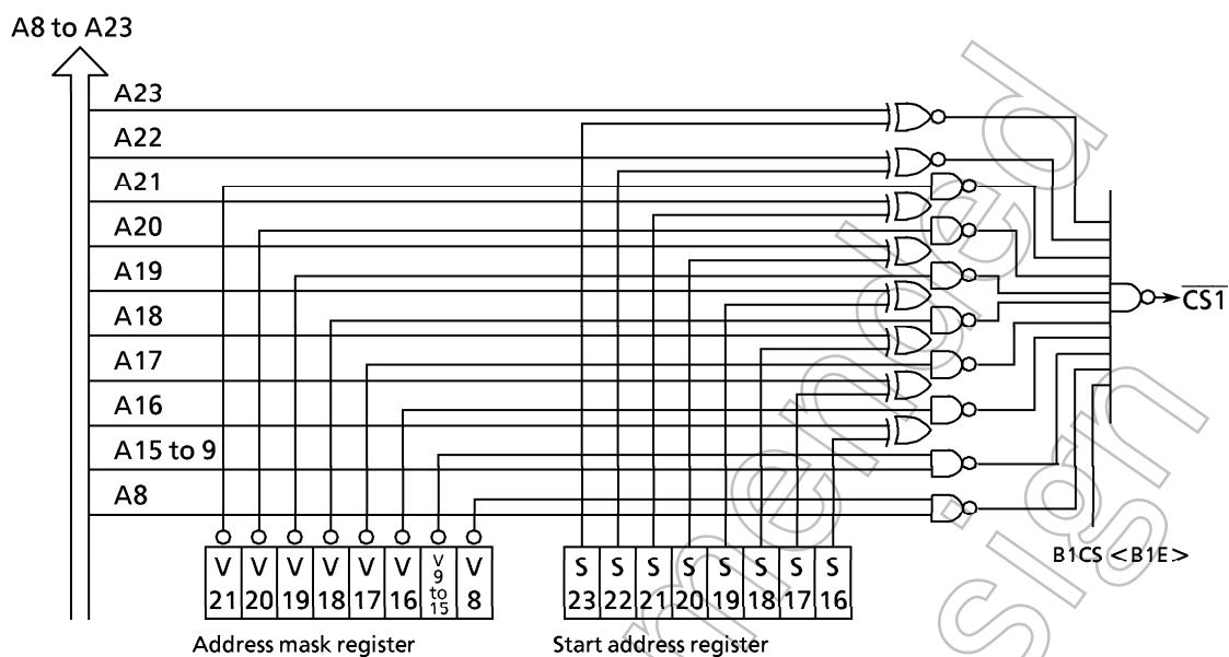
Figure 3.6 (3) \overline{\text{CS1}} Address Decode Block Diagram
