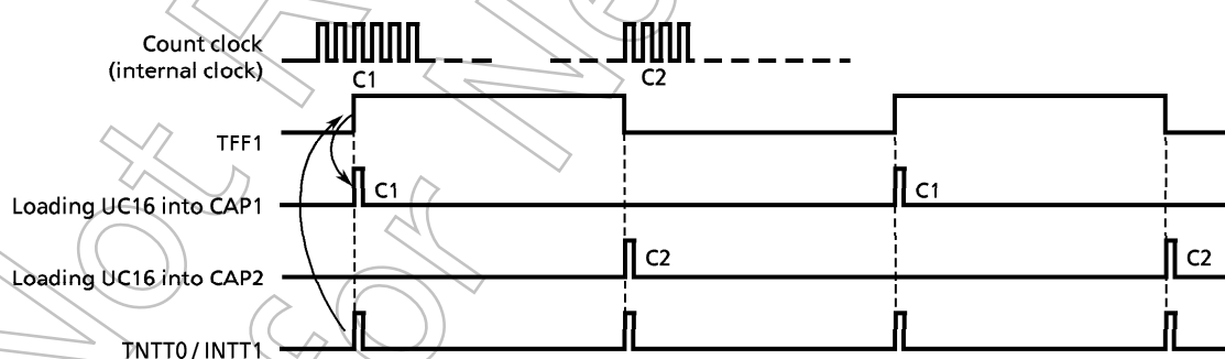
Figure 3.9 (16) Frequency Measurement
