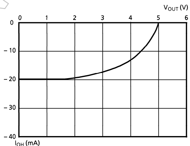
Figure 4.5 V_{OUT} - I_{OH} TYPICAL CURVE
