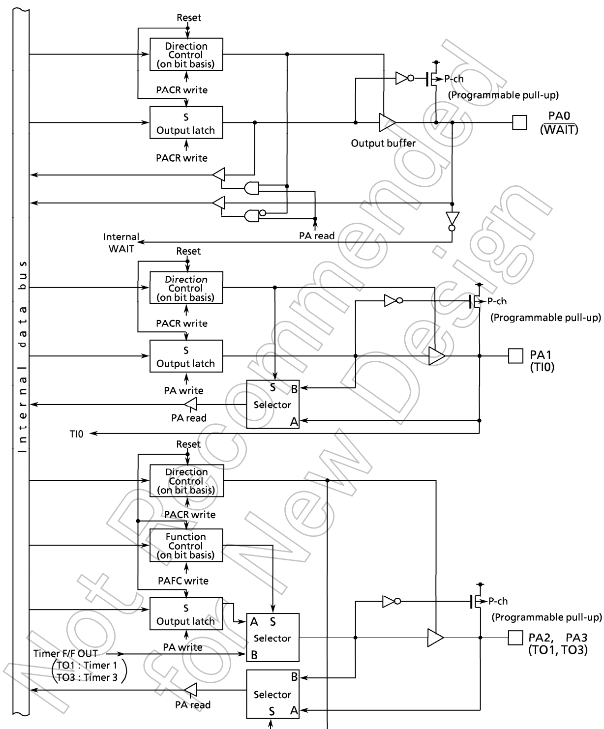
Figure 3.5 (19) Port A
