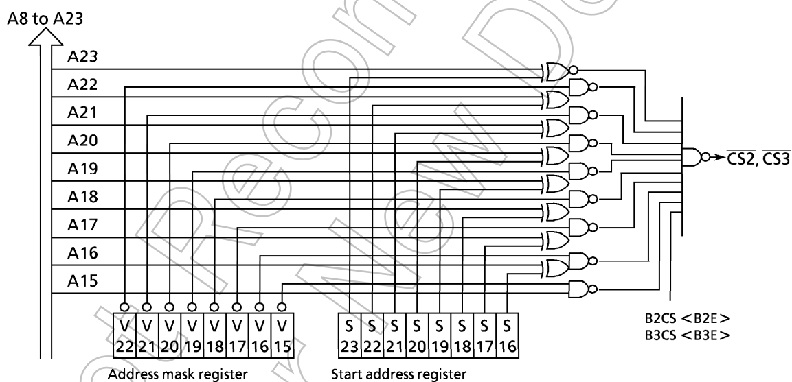
Figure 3.6 (4) \overline{\text{CS2}} \cdot \overline{\text{CS3}} Address Decode Block Diagram
