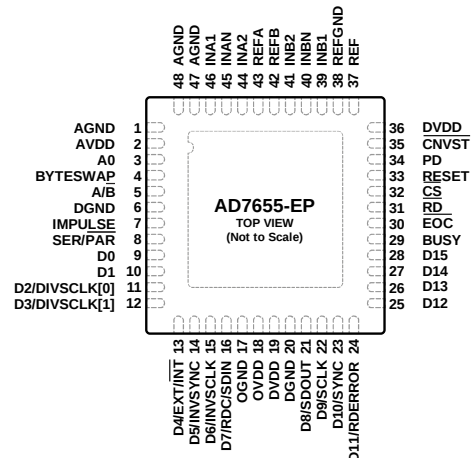
Figure 5. 48-Lead LFCSP (CP-48-4)
