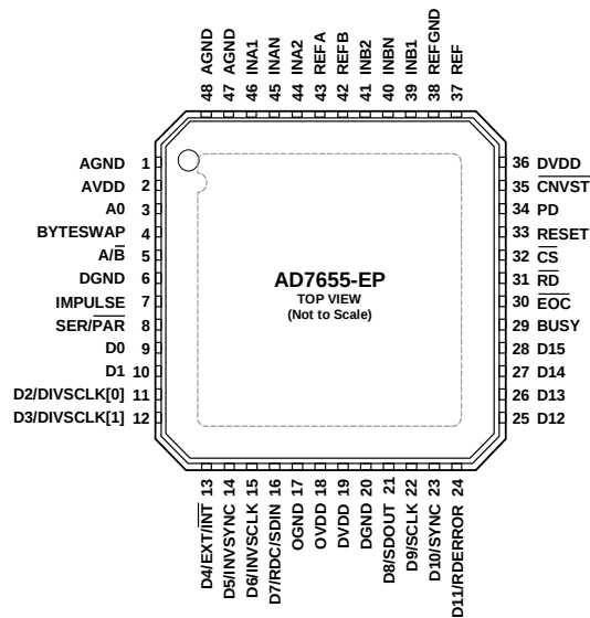
Figure 4. 48-Lead LFCSP (CP-48-1)
