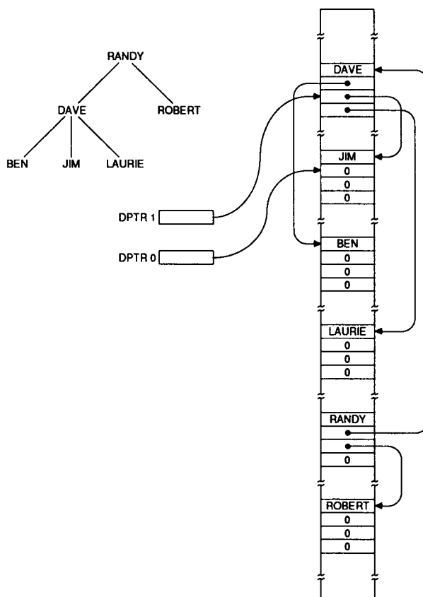
Figure 8-1. Tree Structure in External Memory
